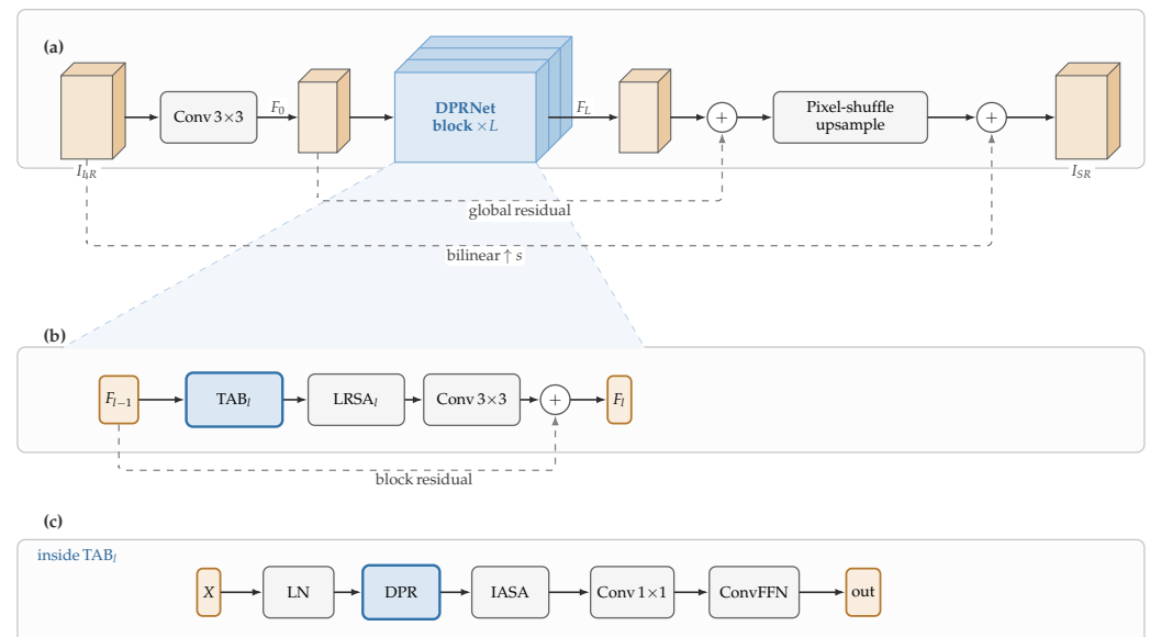
Figure 1. Overall architecture of DPRNet, following the lightweight-SR backbone of CATANet. (a) A 3 \times 3 convolution extracts shallow features F_0 , which pass through a stack of L=8 DPRNet blocks; the deep features are added back through a global residual and reconstructed by a pixel-shuffle upsampler that is summed with a bilinearly upsampled base image. (b) Each block keeps the TAB–LRSA–fusion structure under a residual connection. (c) Inside a TAB, the only modified component is the routing module: DPR replaces center-based routing while preserving the input/output interface, and is expanded in Figure 2.
