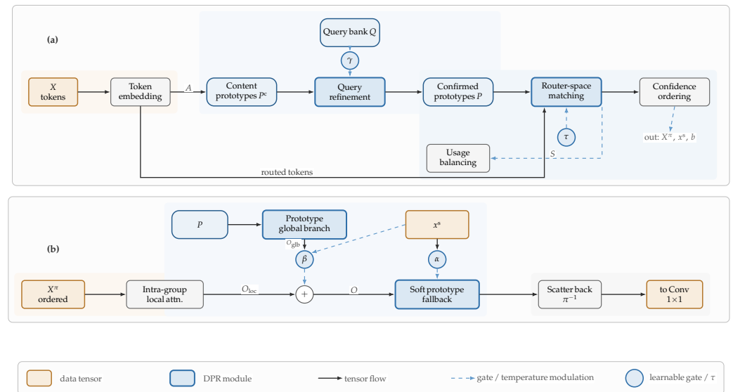
Figure 2. Dynamic Prototype Routing (DPR). (a) The router runs in a single pass: it embeds the tokens, forms content prototypes P^c from the current tokens, confirms them with a learnable query bank through a gated refinement ( \gamma ), and matches the tokens back to the confirmed prototypes P with a bounded temperature \tau , yielding the ordered sequence X^\pi , the confidence x^s , and the label b (Eqs. (4)–(10)); the usage-balancing term acts on the score map S (Eq. (13)). (b) IASA consumes X^\pi , P , and x^s : a local branch and a prototype global branch are combined under a confidence-modulated gate \beta , and a soft prototype fallback gated by \alpha stabilizes low-confidence tokens before the output is scattered back via \pi^{-1} (Eqs. (11)–(12)).
