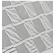
CATANet
