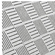
GT
