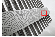
Urban100: img_092
