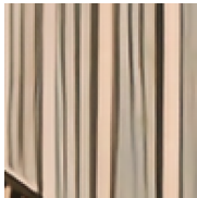
SRFormer-light
