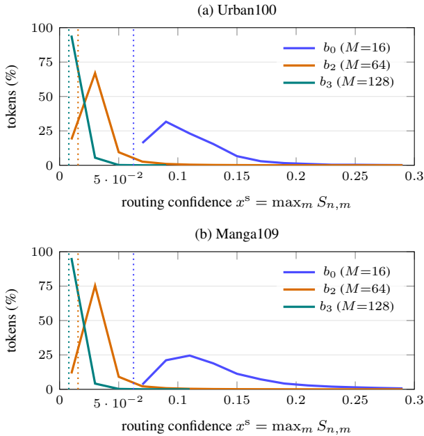
Figure 5. Distribution of the per-token routing confidence x^s = \max_m S_{n,m} (Eq. (9)) at \times 4 , accumulated over all test images of (a) Urban100 and (b) Manga109 with the final model. Curves are shown for three representative TAB blocks with increasing prototype count M ; dotted vertical lines mark the uniform-assignment floor 1/M . In every plotted block the distribution sits clearly to the right of its floor (block means are about 1.5–2.1 times 1/M ) yet stays far from 1, confirming that the softmax assignment is informative but soft : tokens commit to a prototype more than chance while retaining the graded confidence that the C3 components (ordering key, IASA gate, soft fallback) rely on. As M grows the mode shifts toward the (lower) floor, consistent with confidence being spread over more slots.
