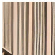
SwinIR-light
