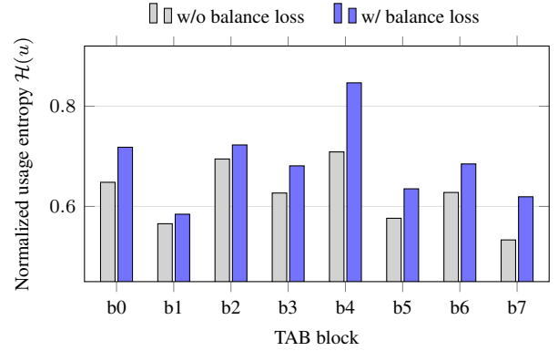
Figure 1. Normalized prototype-usage entropy \mathcal{H}(u) (Eq. (13); higher = more balanced) per TAB block ( b_0 – b_7 ) at \times 4 , iter 80k on Urban100. The usage-balancing regularizer increases the entropy in all eight blocks (block-mean 0.6227 \rightarrow 0.6865), confirming that it counteracts the collapse onto a few prototypes encouraged by the learnable temperature (C4).
