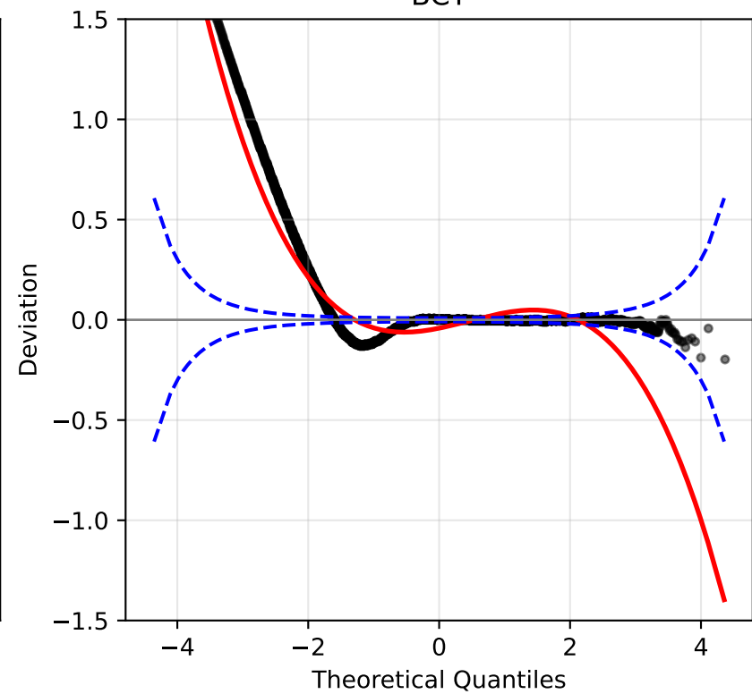
BCT
