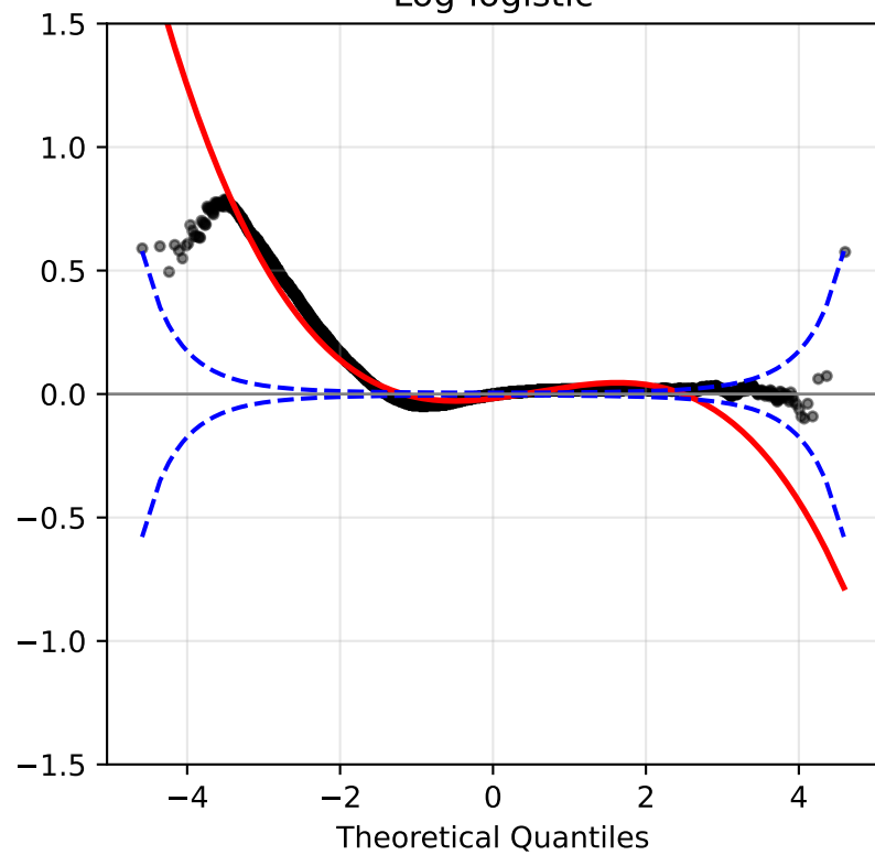
Log-logistic
