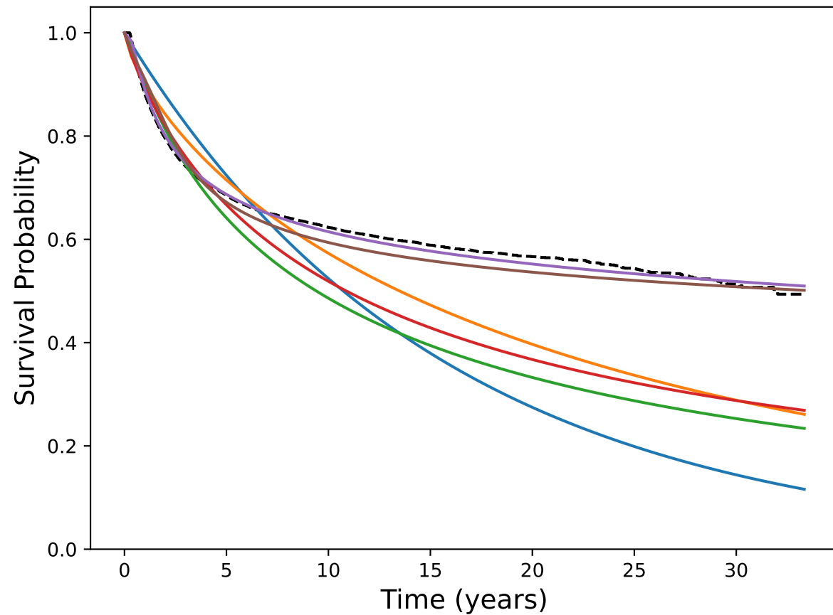
(a) Without covariates
