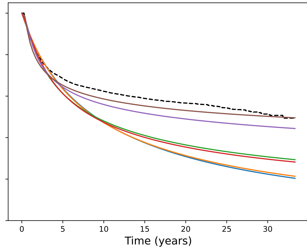
(b) With covariates
