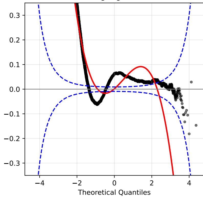
Log-logistic
