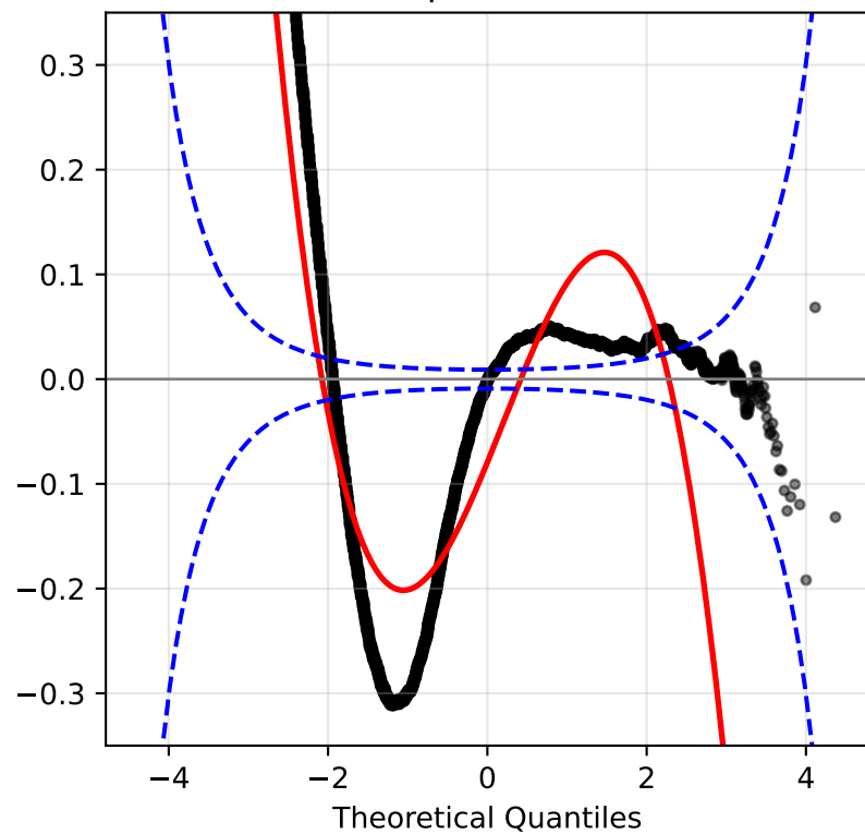
Log-logistic
