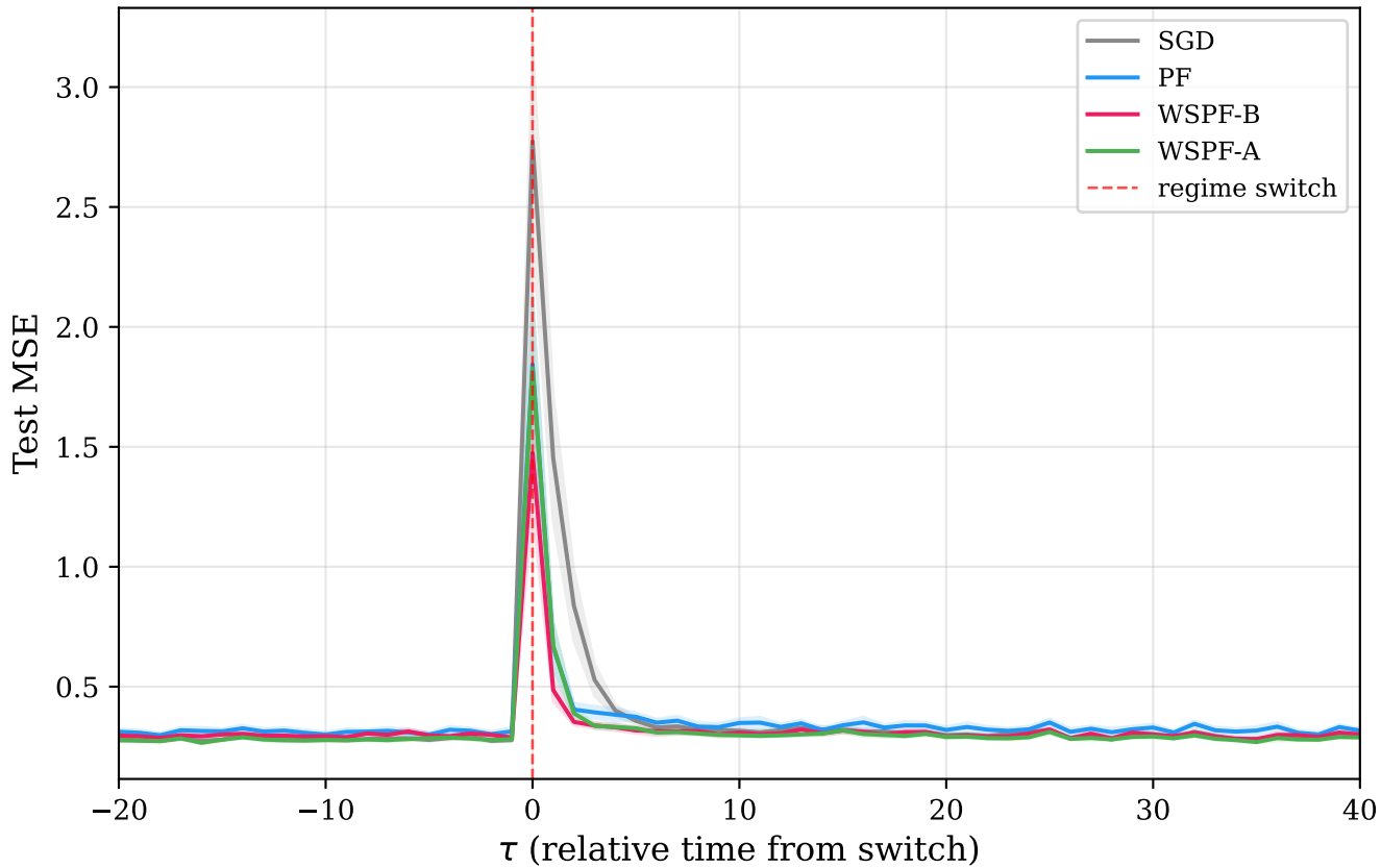
Switch-Aligned Recovery: Test MSE around regime changes
