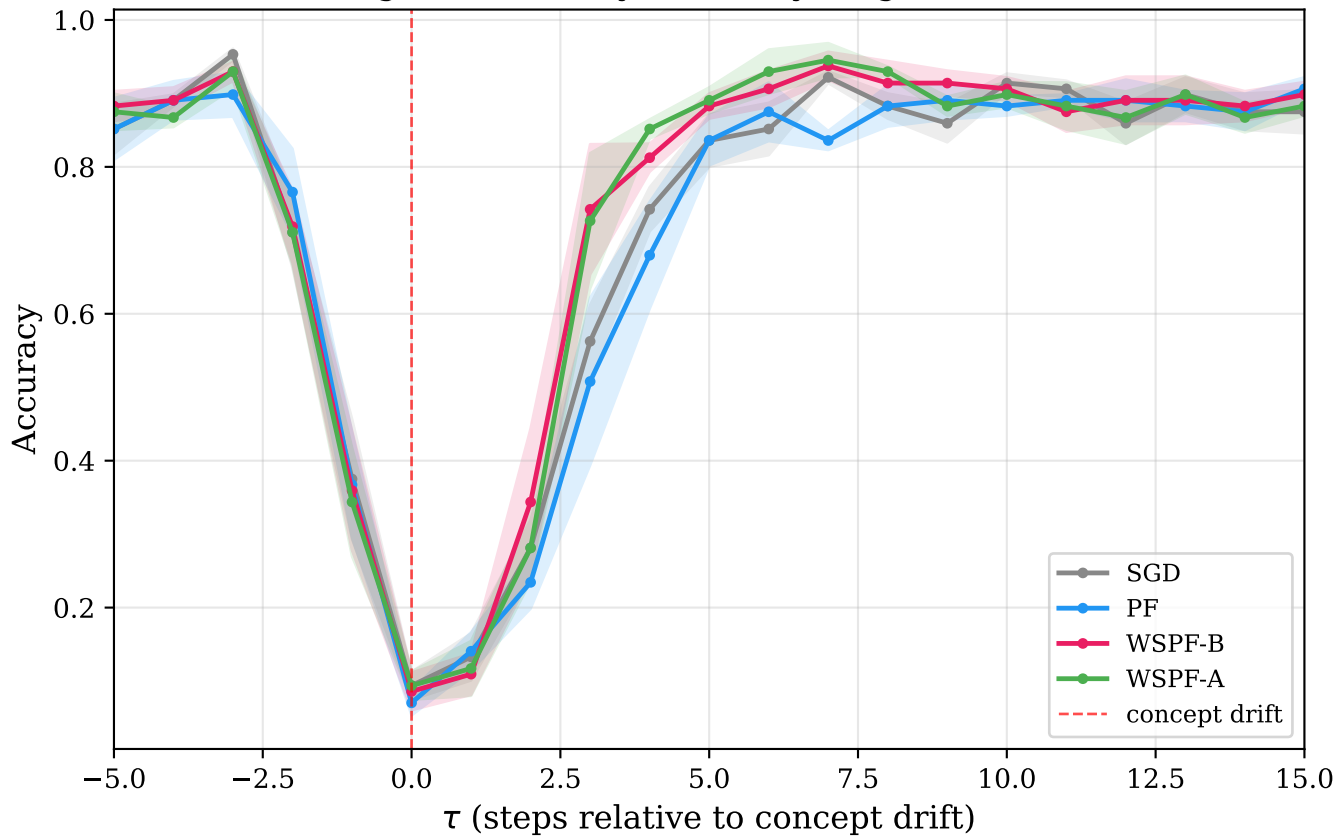
Email: Switch-Aligned Accuracy Recovery (avg over 4 switches, N=100)
