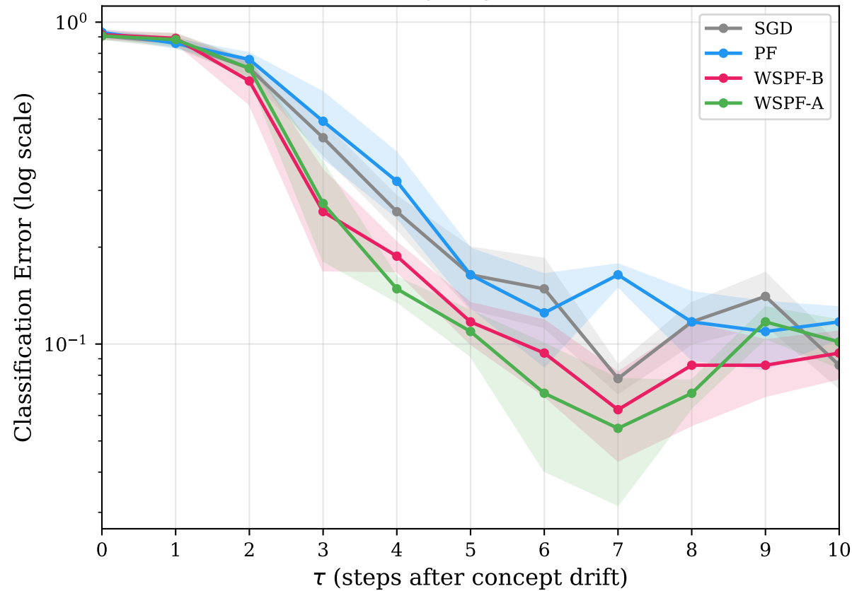
Email: Post-Switch Recovery (log scale, first 10 steps, N=100)
