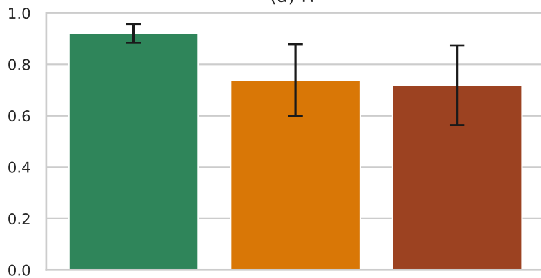
(a) R^2
