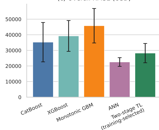
(c) Overall RMSE (USD)
