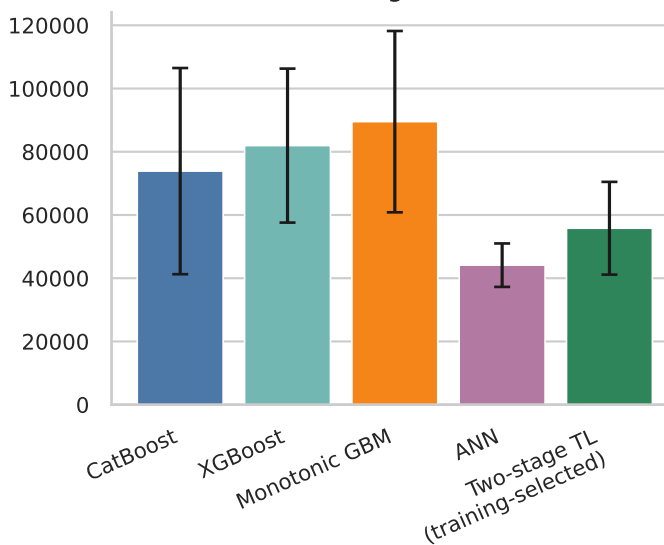
(e) RMSE \geq \text{training Q3} + IQR/2 (USD)
