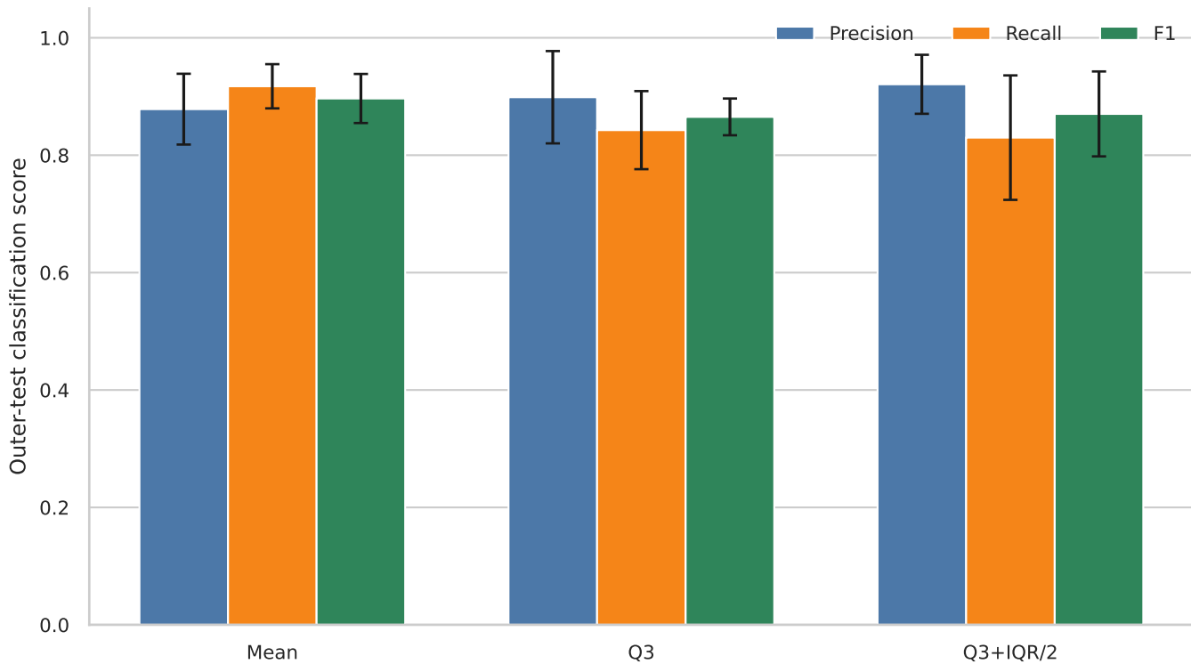
SVM classification under training-derived cutoffs
