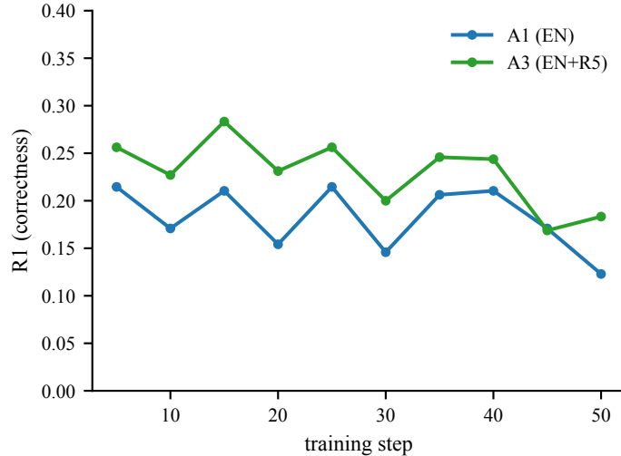
R1: Correctness reward
