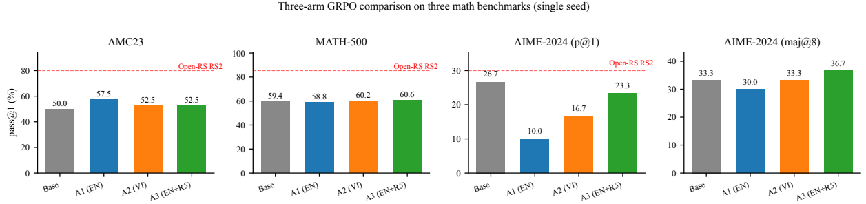
Fig. 1. Three-arm GRPO comparison on three mathematical reasoning benchmarks (single seed, seed=42 ). Bar height denotes pass@1 except for the rightmost panel which is maj@8. The red dashed line shows the Open-RS RS2 reported value [3]; the residual gap between our base and Open-RS reported reflects evaluation-pipeline differences discussed in Section VIII.
