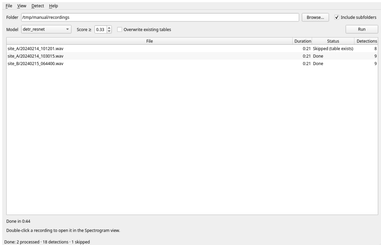
Figure 4: Batch after a run: one file skipped (it had a table), two done.
