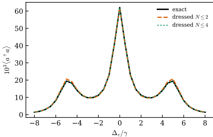
Mollow triplet seen by the cavity
