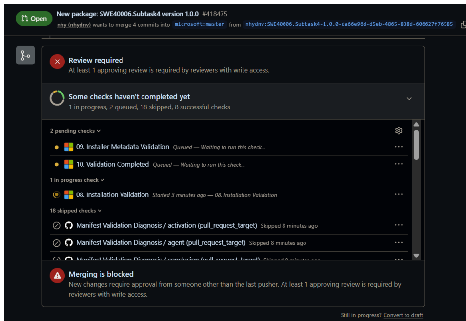
Figure 33: The WinGet validator checking the contents of my pull request before merging it to the master branch.
