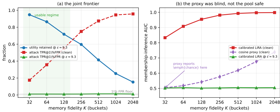
Fig. 1 (a) The joint frontier. Utility retention falls monotonically with fidelity K while clean leakage rises; DP pins the calibrated attack at the 1% false-positive floor uniformly , so the frontier is governed by the utility axis alone and the coarse- K regime dominates. (b) Why the superseded draft missed this. The uncalibrated cosine proxy (purple) reports chance at K = 32 on the same clean release where the calibrated LiRA (red) reads AUC 0.833. The proxy was blind; the pool was not safe (§7.5).
