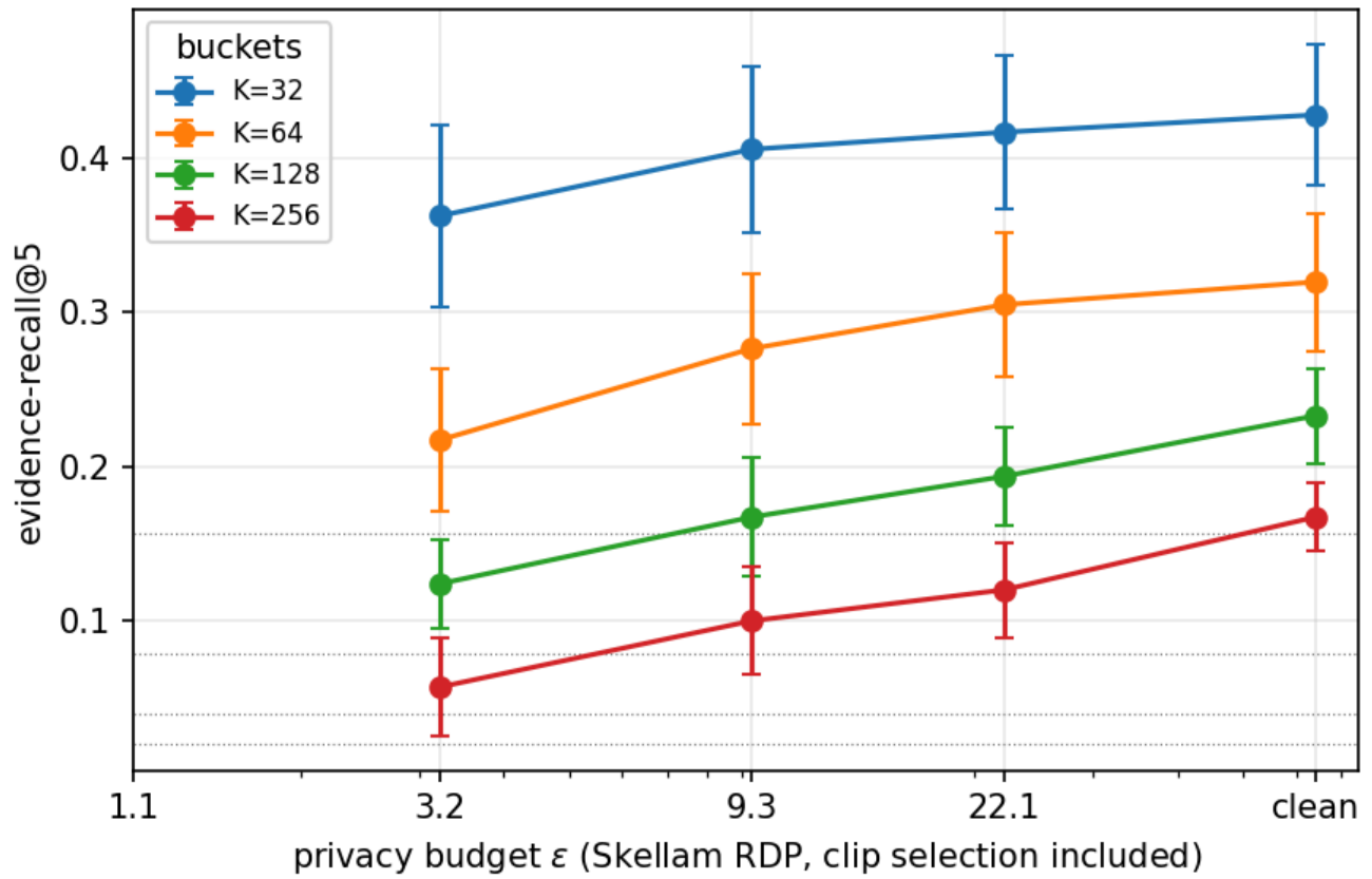
LongMemEval oracle: DP utility holds at tiny-K
