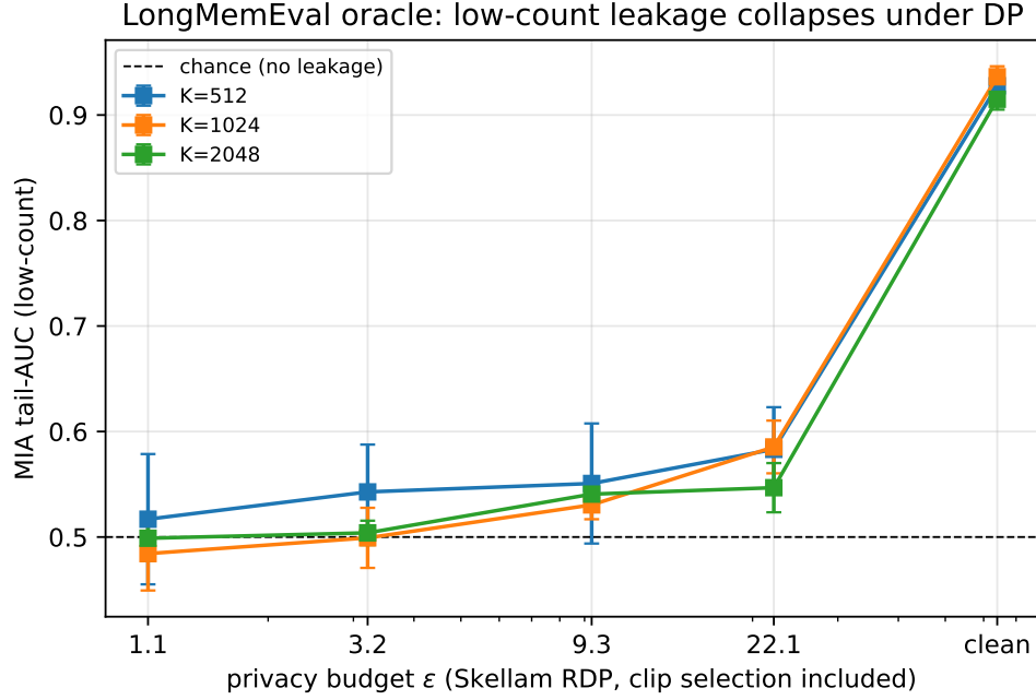
Fig. 4 The proxy’s own endpoint, retained for the record: on the sparse tail it can see ( K \geq 512 ), membership-inference AUC falls from \approx 0.93 to 0.53\text{--}0.55 at \epsilon \approx 9.3 . The result is real but the lens is narrow: at K \leq 128 this tail is empty and the proxy reports chance, while the calibrated attack of §7.3 shows the release is leaking there too (Fig. 1b).
