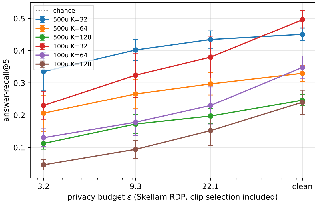
Distilled-notes utility: density lifts DP retention (500u vs 100u)
