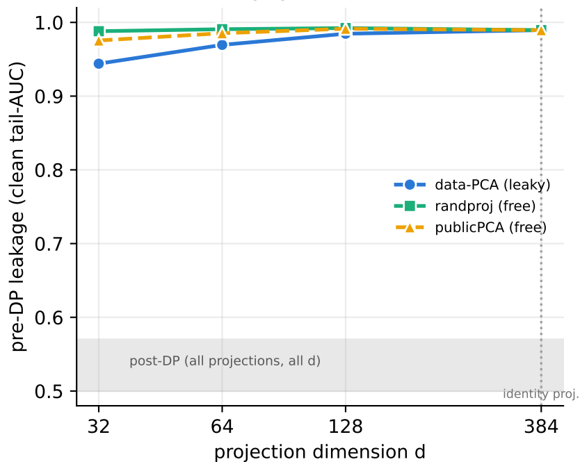
(b) the leakage gradient is an artifact too
