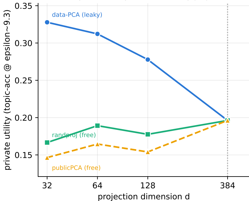
(a) tiny-d wins only under the leaky projection
