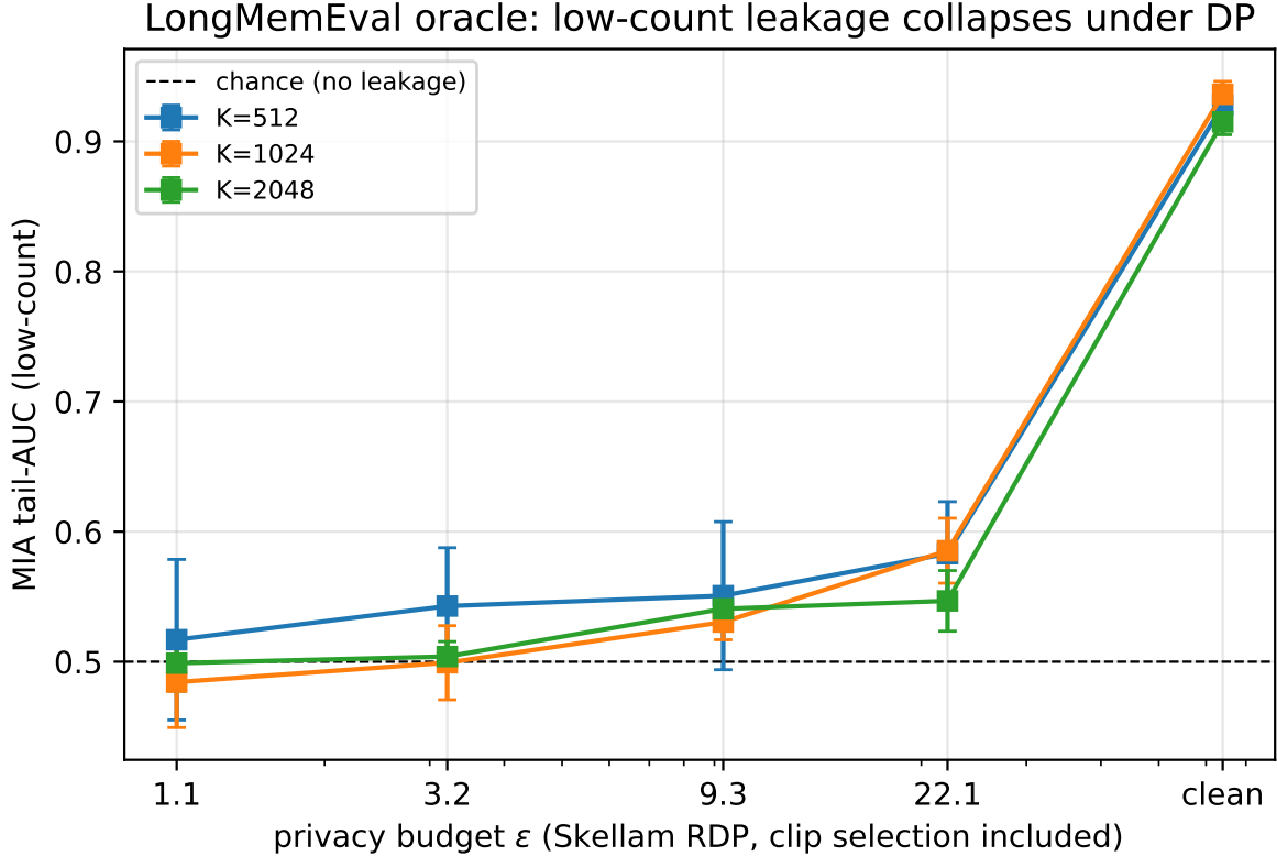
Fig. 4 The proxy’s own endpoint, retained for the record: on the sparse tail it can see ( K \geq 512 ), membership-inference AUC falls from \approx 0.93 to 0.53–0.55 at \varepsilon \approx 9.3 . The result is real but the lens is narrow: at K \leq 128 this tail is empty and the proxy reports chance, while the calibrated attack of §7.3 shows the release is leaking there too (Fig. 1b).
