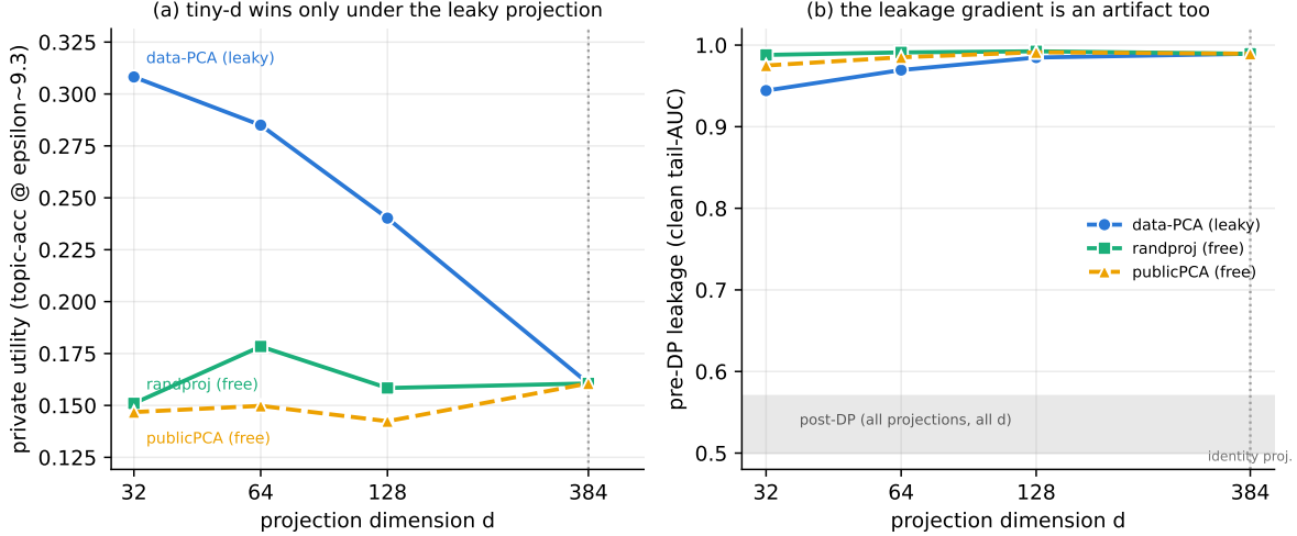
Fig. 3 The dimension crossover is a property of the projection, not of the mechanism. (a) Private utility: tiny- d wins only under the data-dependent PCA; under either data-independent projection it is the worst choice. (b) Pre-DP leakage: data-PCA shows the rising gradient the crossover claim rested on; the honest projections are saturated. All three converge at d = 384 , where the projection is the identity: the control. Shaded band: post-DP tail-AUC, flat at chance for every d and every projection.
