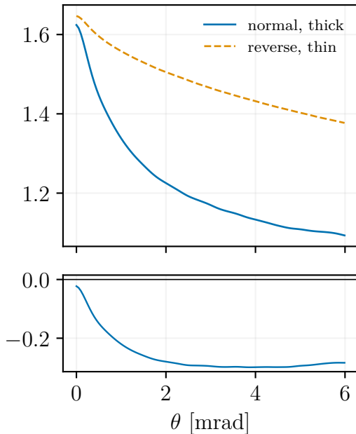
(b) 35 nm homogeneous
