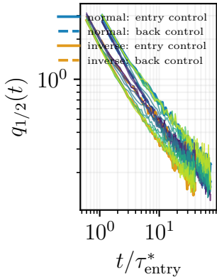
(a) gated cone width
