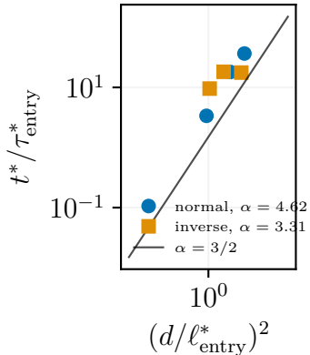
(c) break time
