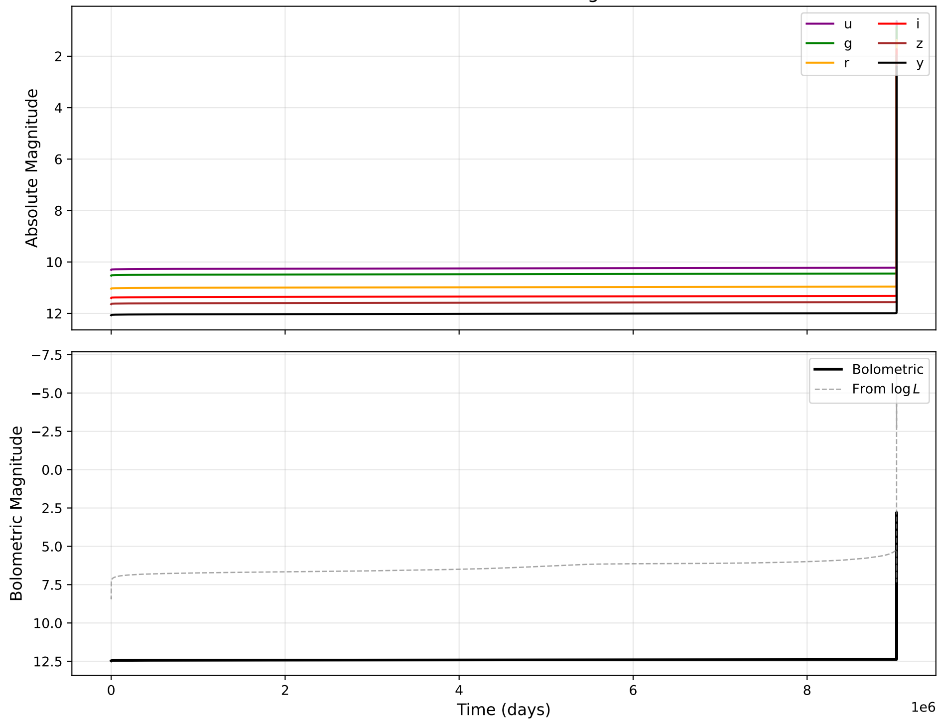
Nova Outburst: Multi-band Light Curves
