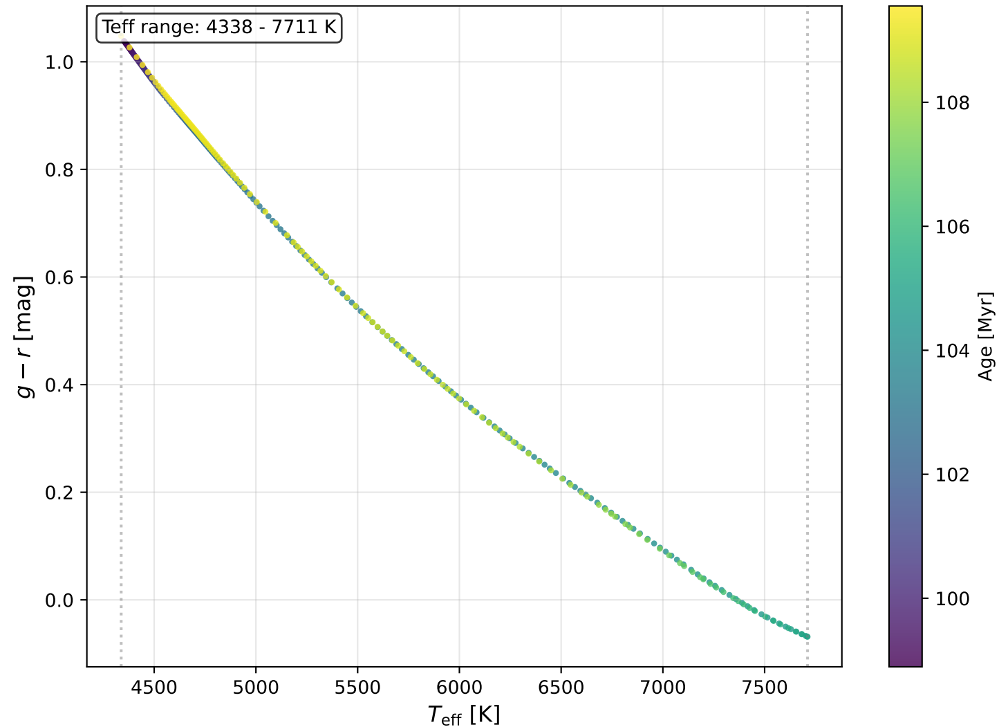
Color-Temperature Relation During Blue Loop
