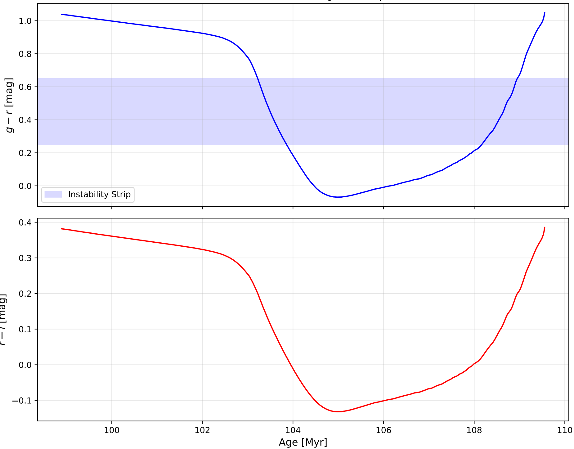
Color Evolution During Blue Loop
