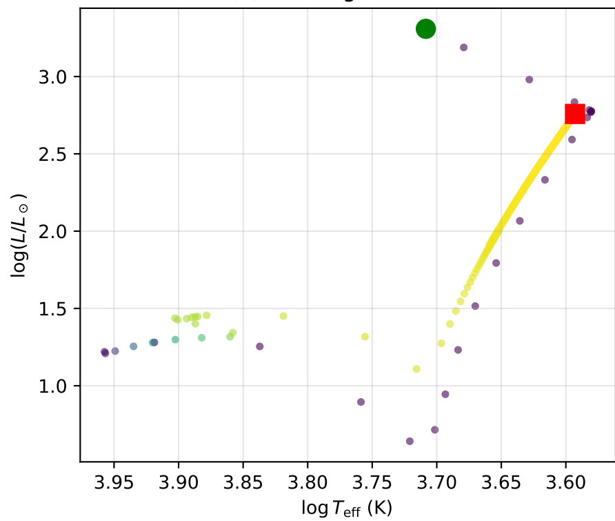
(c) HR Diagram Track
