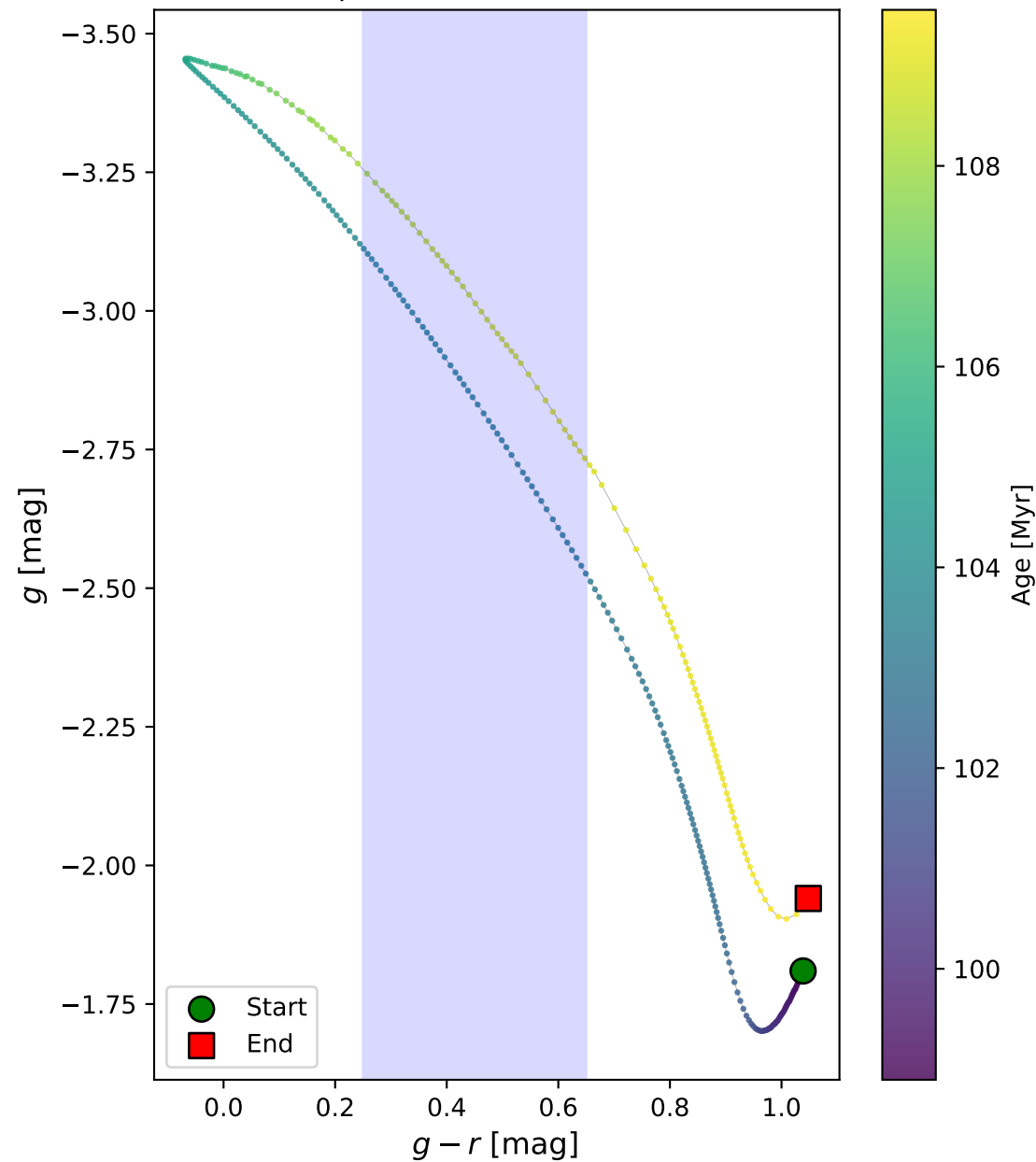
Blue Loop CMD Track (LSST filters, AB)
