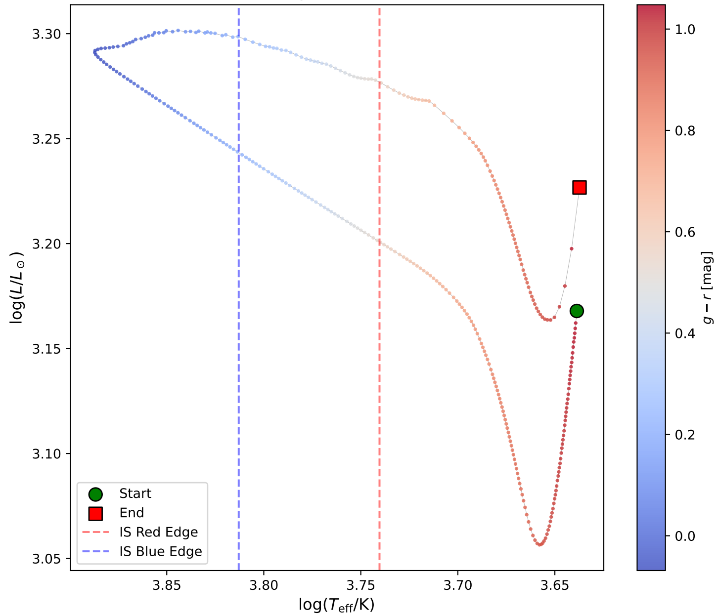
HR Diagram with Colors
