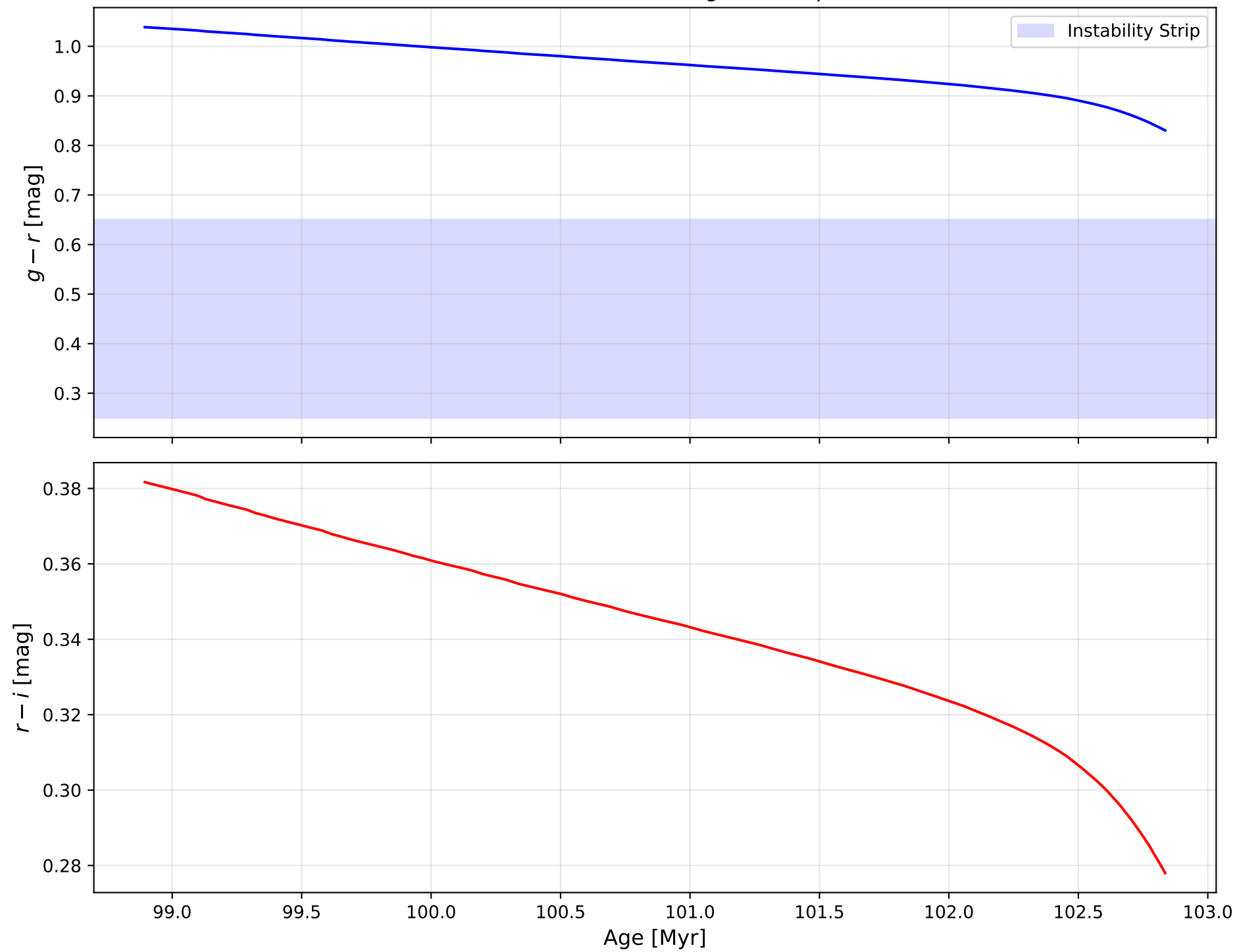
Color Evolution During Blue Loop
