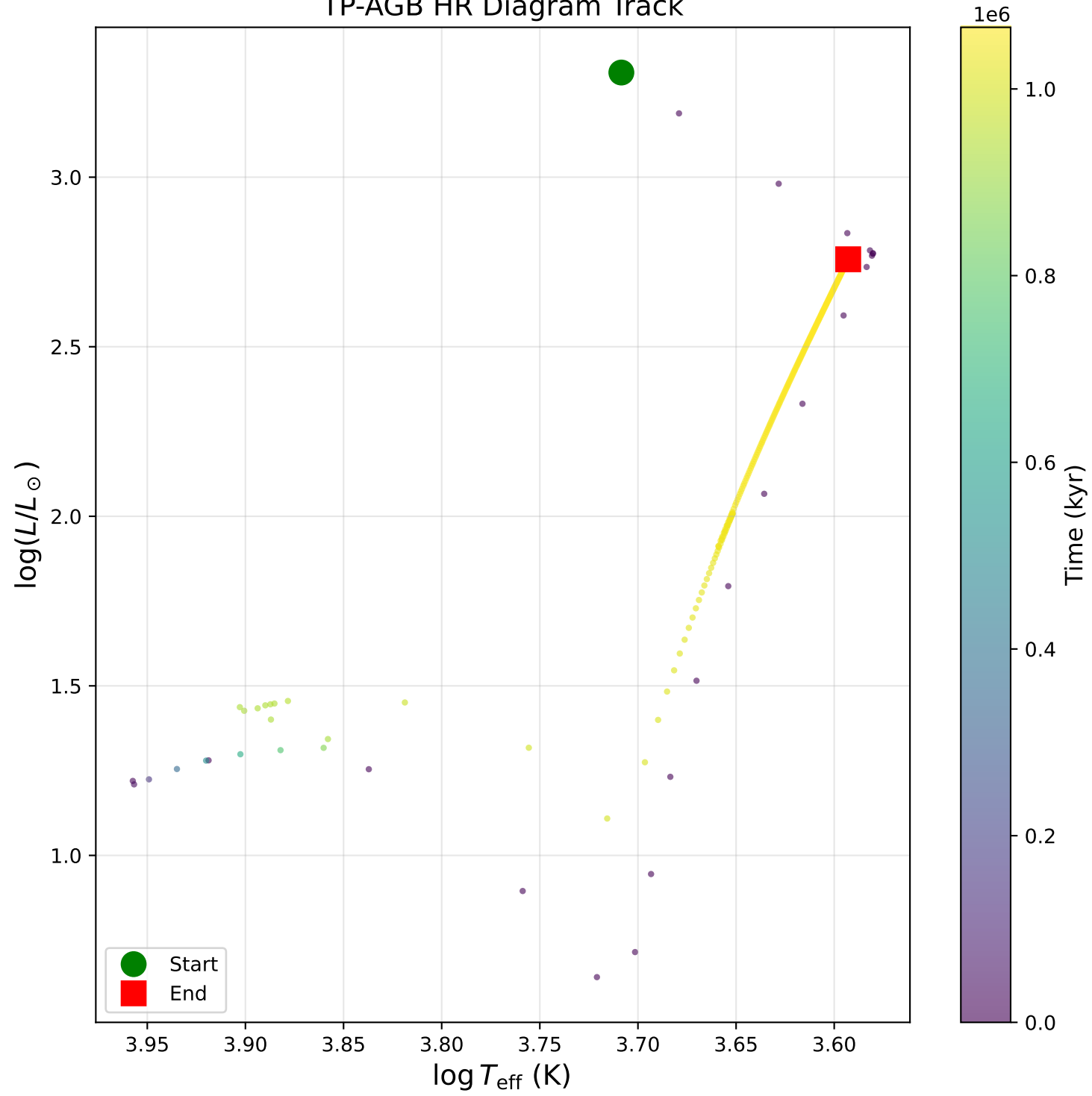
TP-AGB HR Diagram Track
