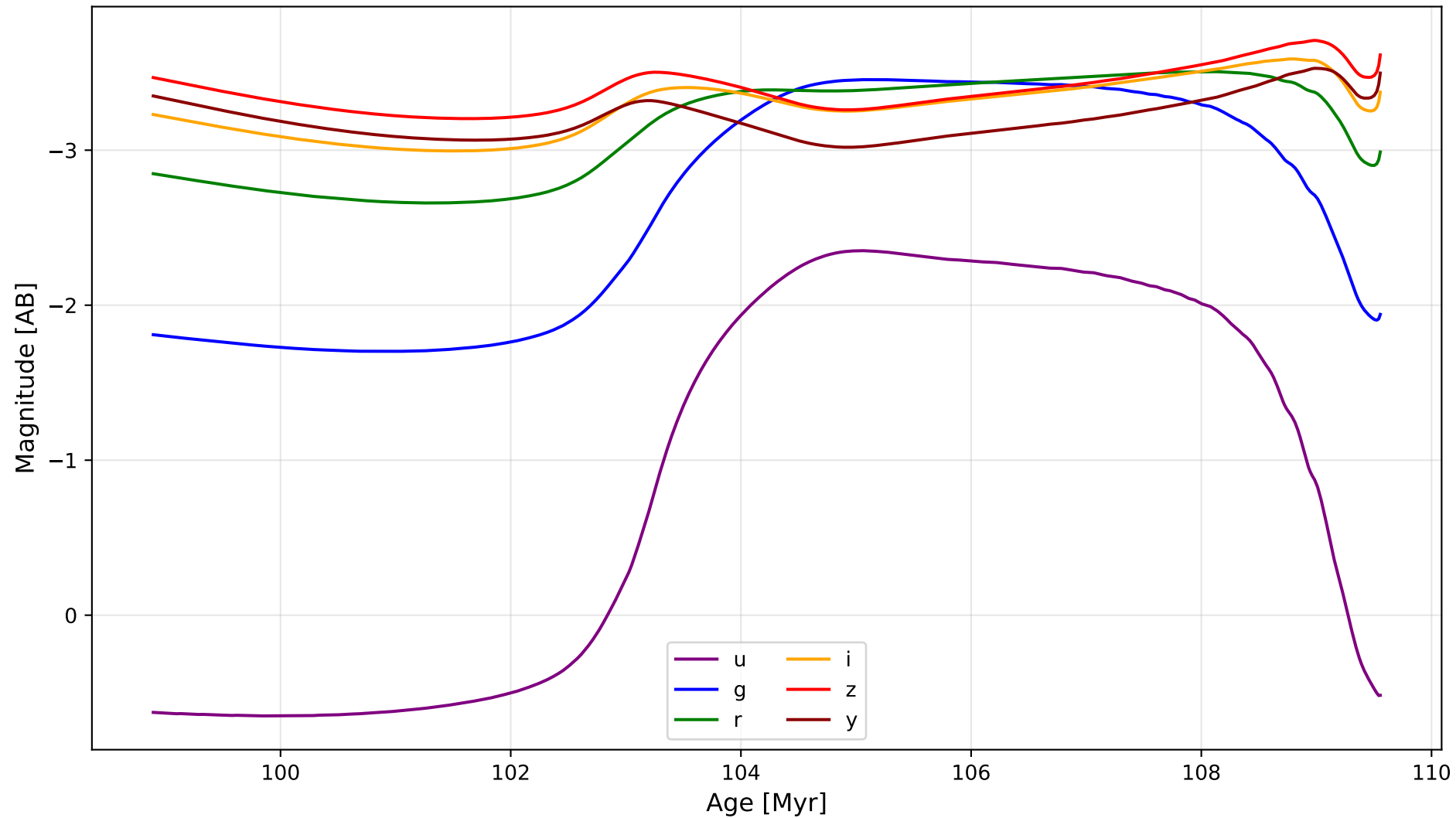
Multi-band Magnitude Evolution During Blue Loop
