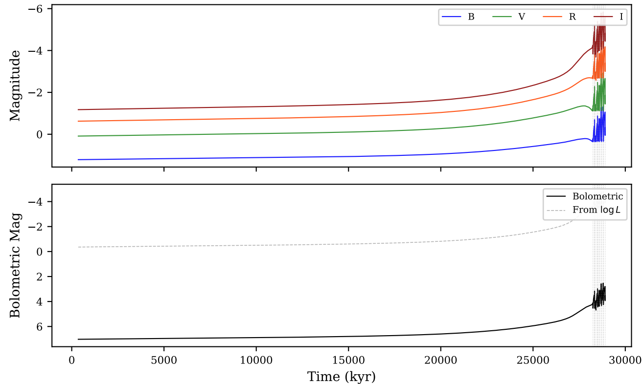
TP-AGB Evolution (13 thermal pulses)
