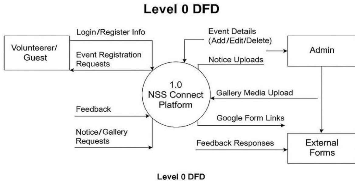
Fig 5.4.1 Data Flow Diagram - Level 0
