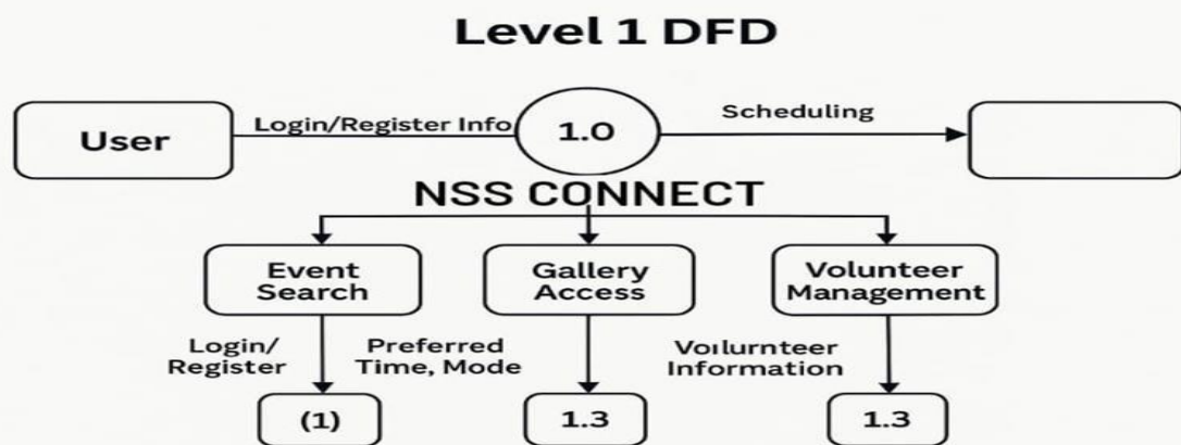
Fig 5.4.2 Data Flow Diagram – Level 1
