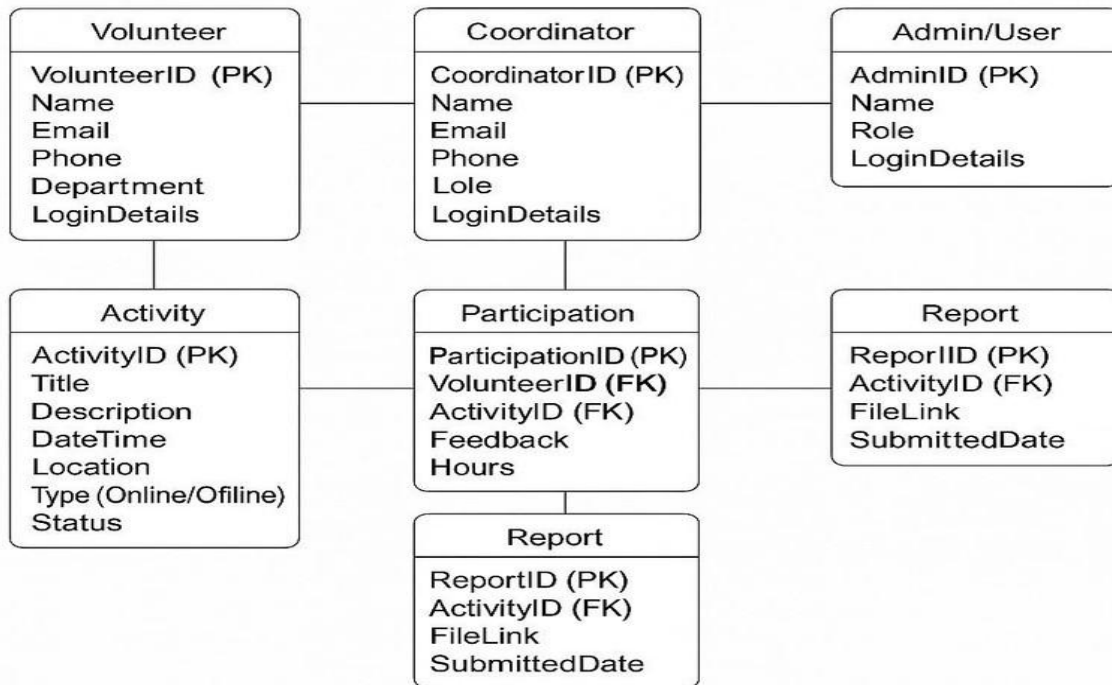
Fig 5.5 Entity Relationship Diagram
