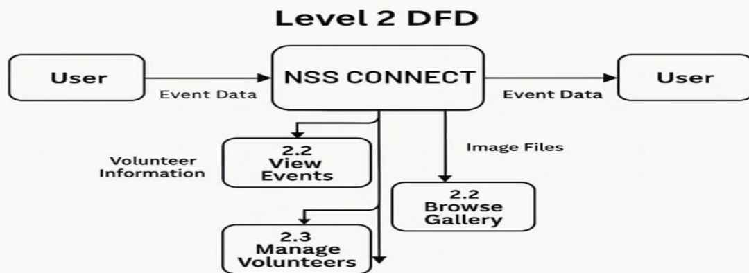
Fig 5.4.3 Data Flow Diagram – Level 2
