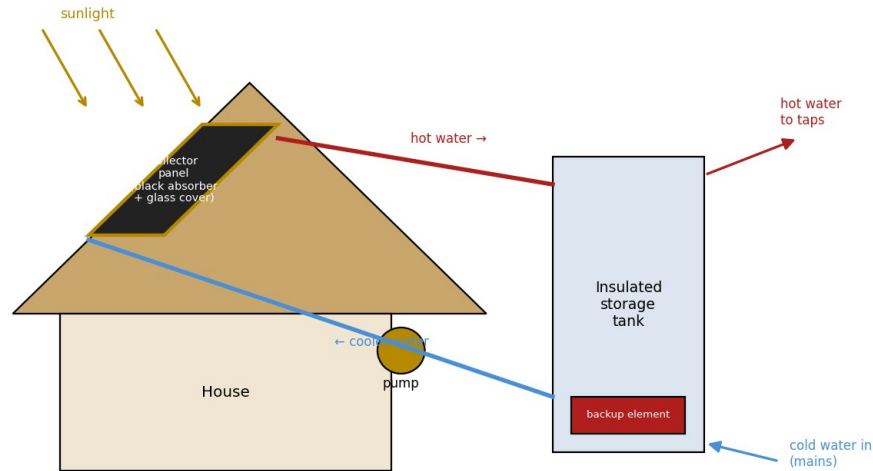
A domestic solar water heater
