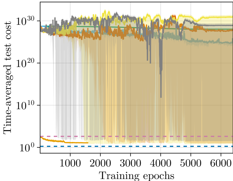
LSTM
