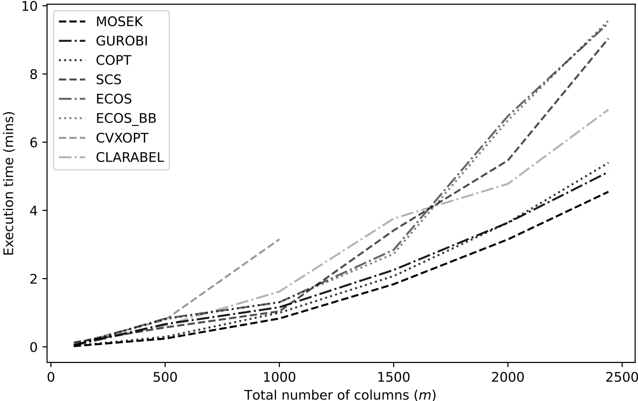
Solvers mean execution times for the SOCP problem
