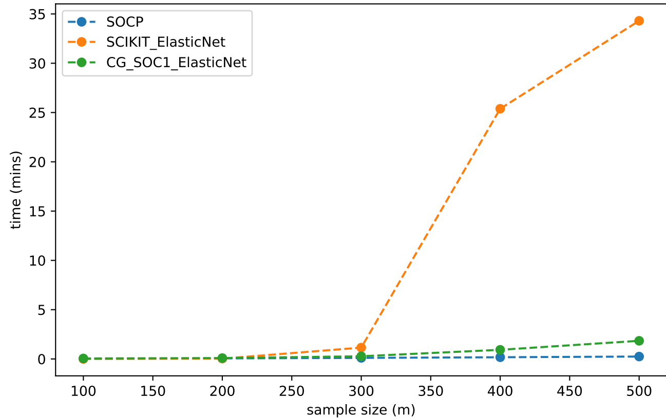
Execution times as a function of the sample size (m)
