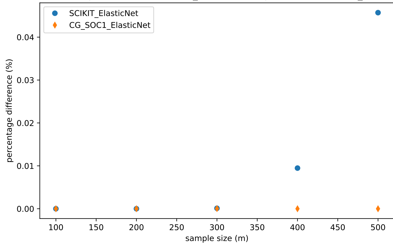
Percentage difference of the fo_value with respect to the SOCP fo_value
