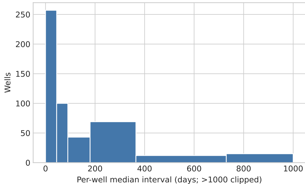
Observation cadence
