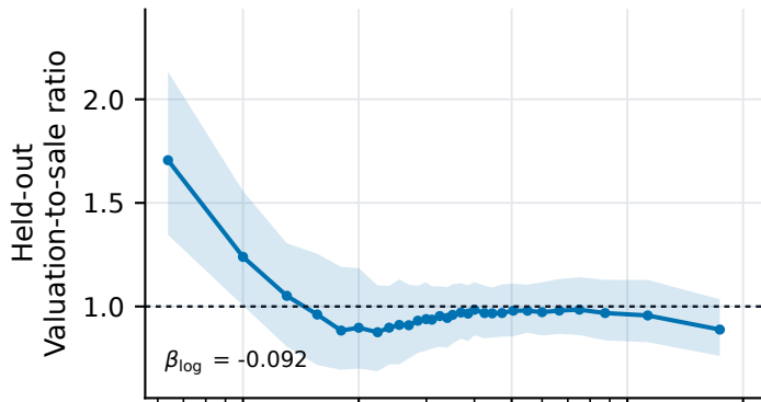
Ordinary linear regression
