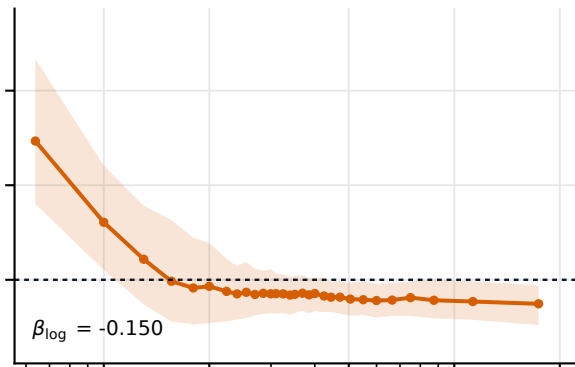
Ordinary LightGBM
