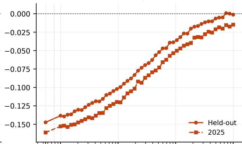
Surrogate
