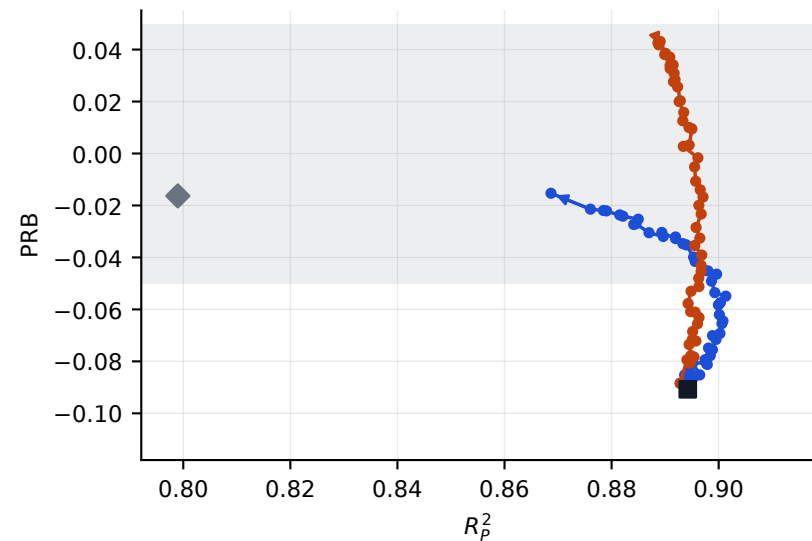
Held-out: PRB
