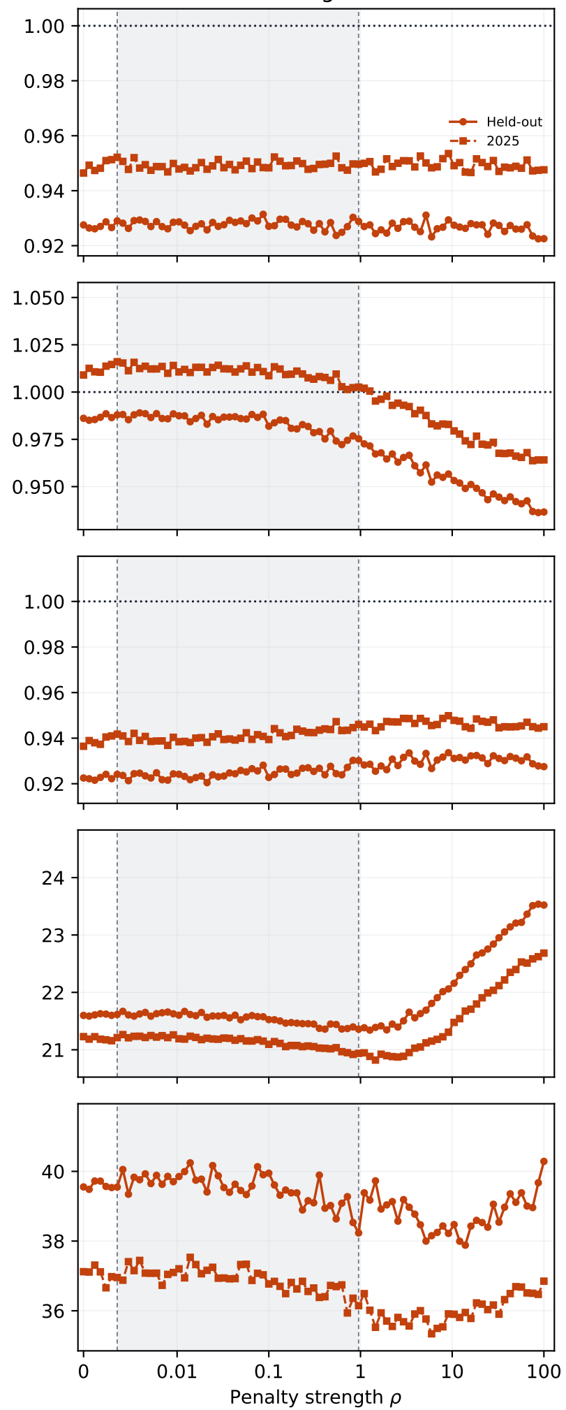
Surrogate
