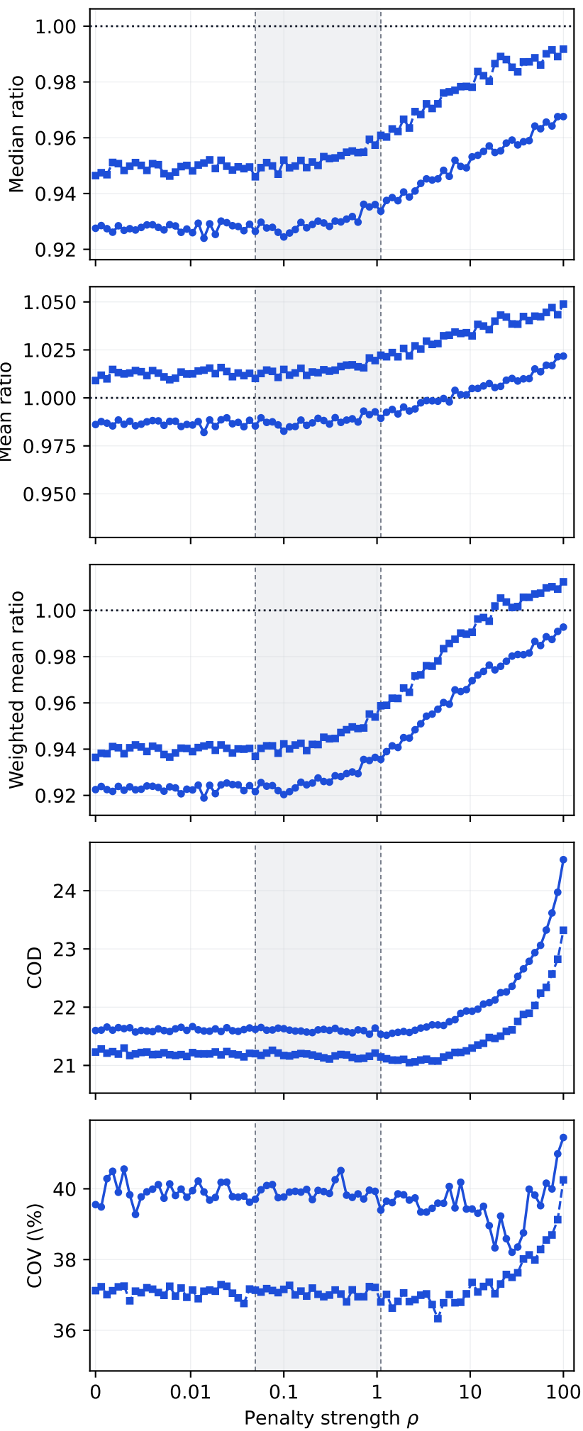
Direct
