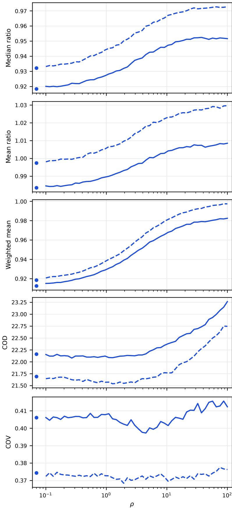
Direct
