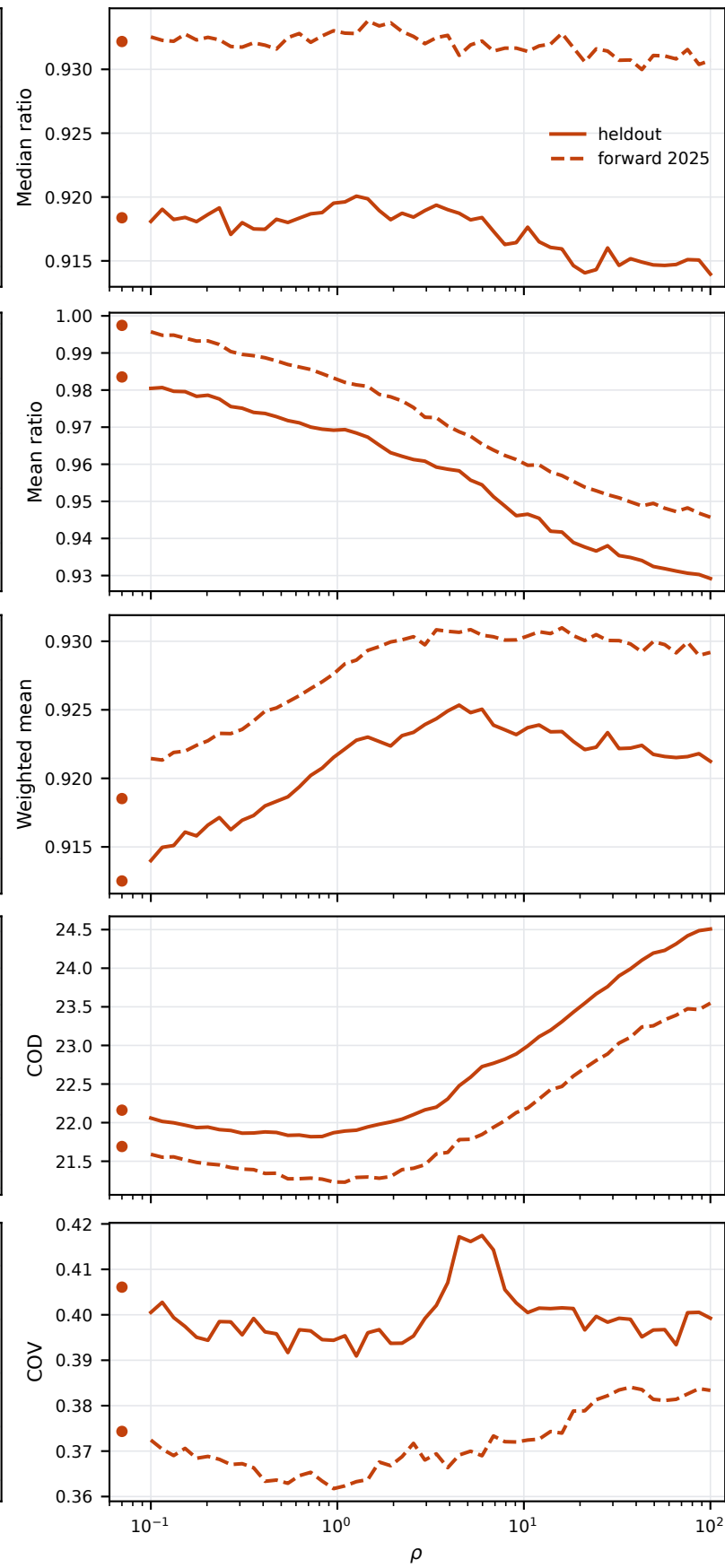
Surrogate
