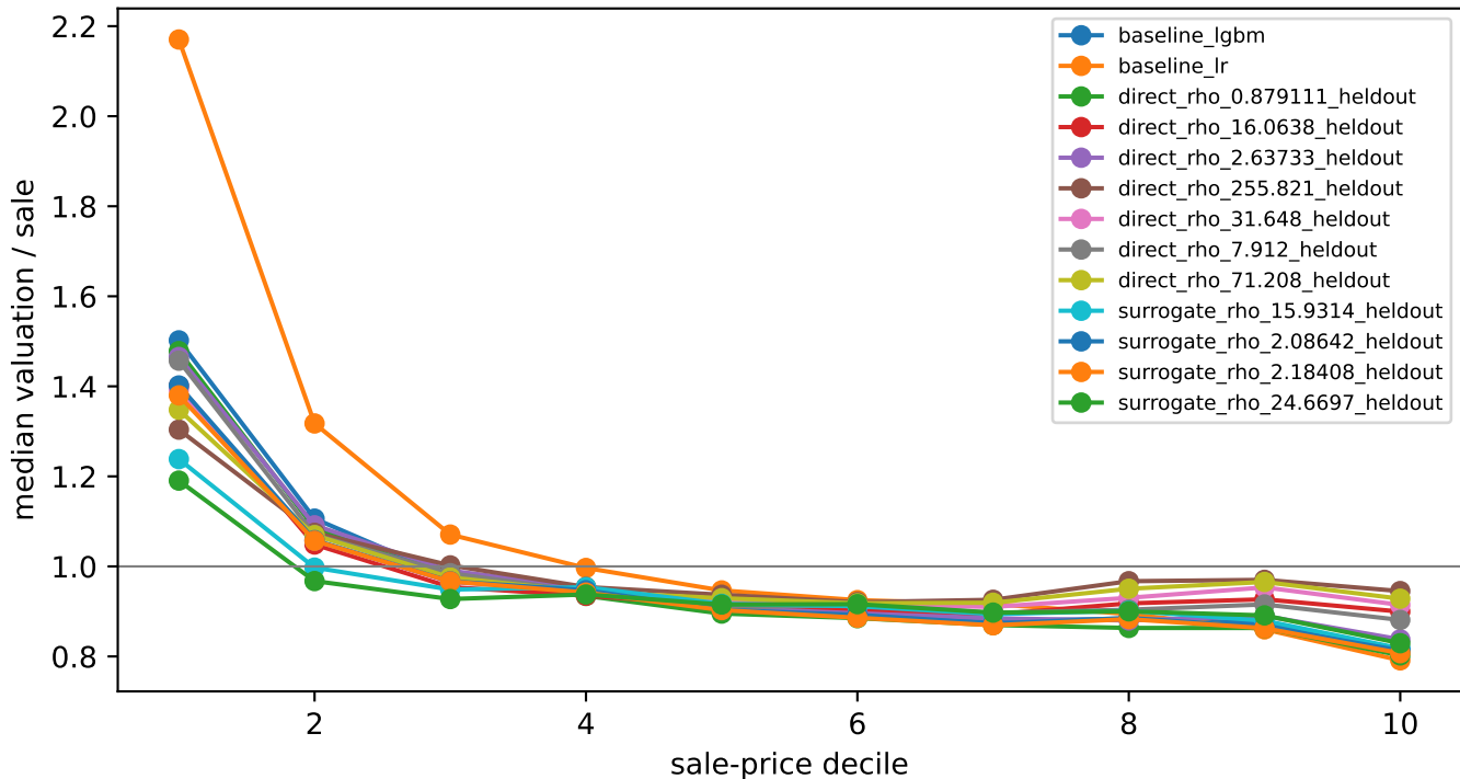
philadelphia held-out ratio profiles
