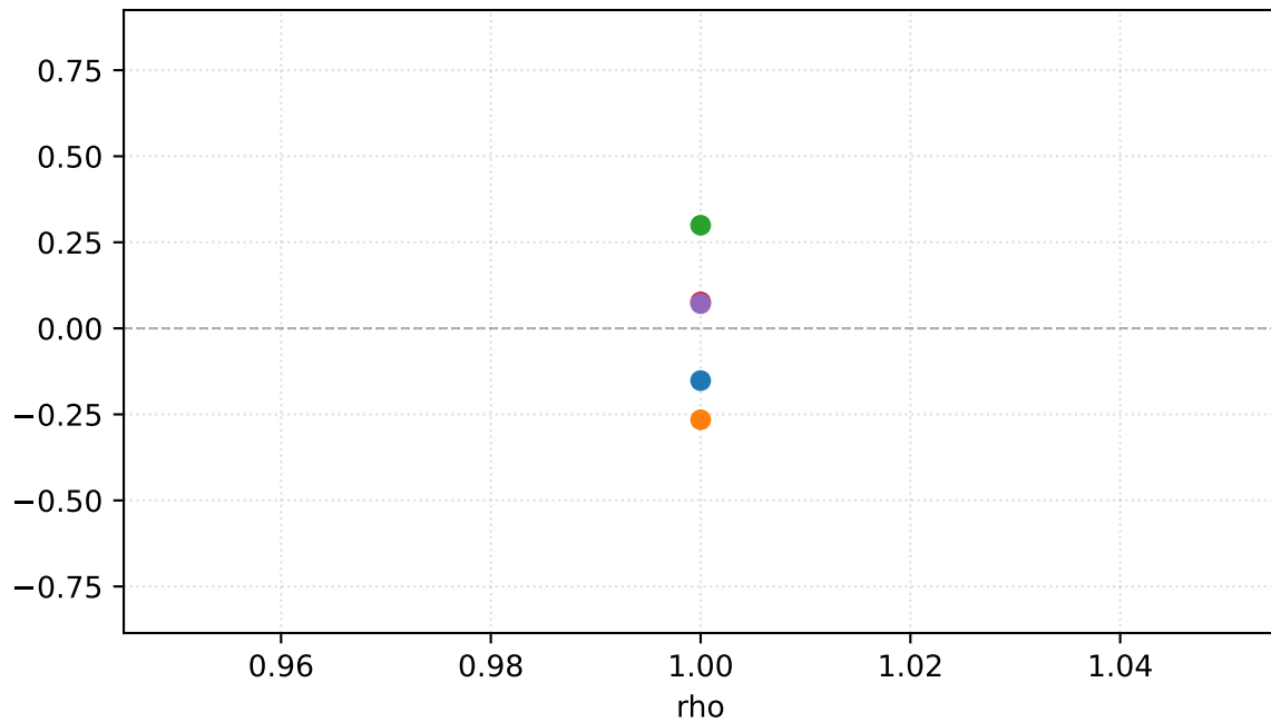
LGBSmoothPenalty
