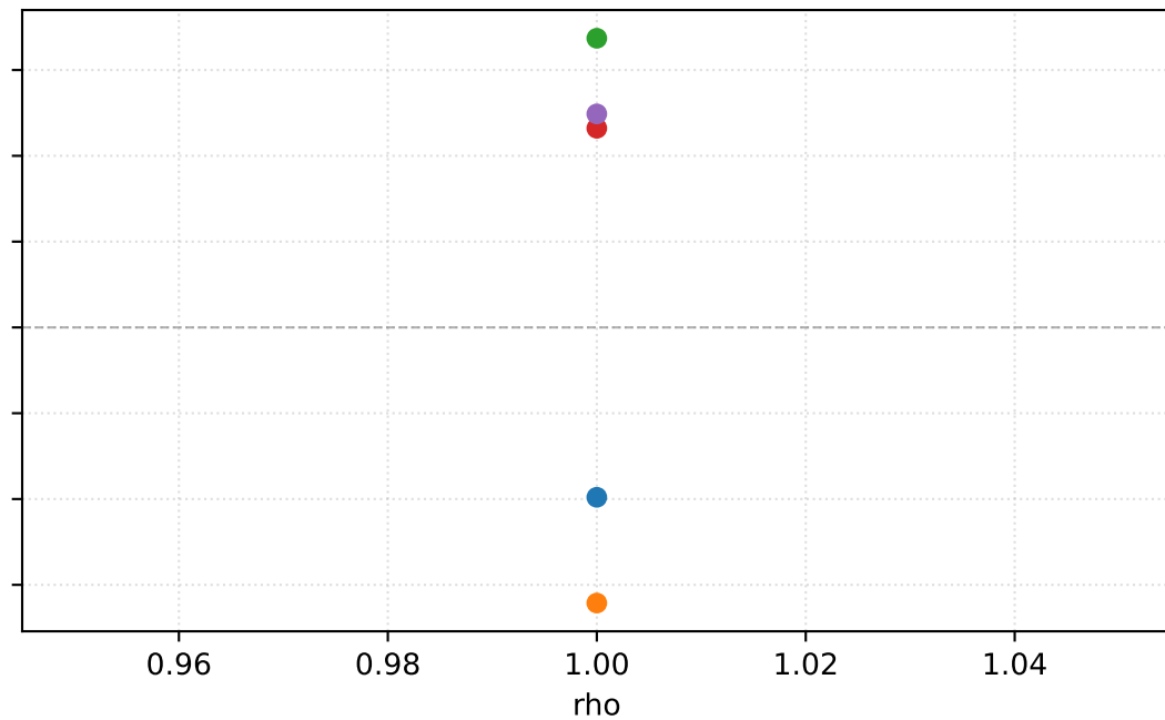
LGBCovPenalty
