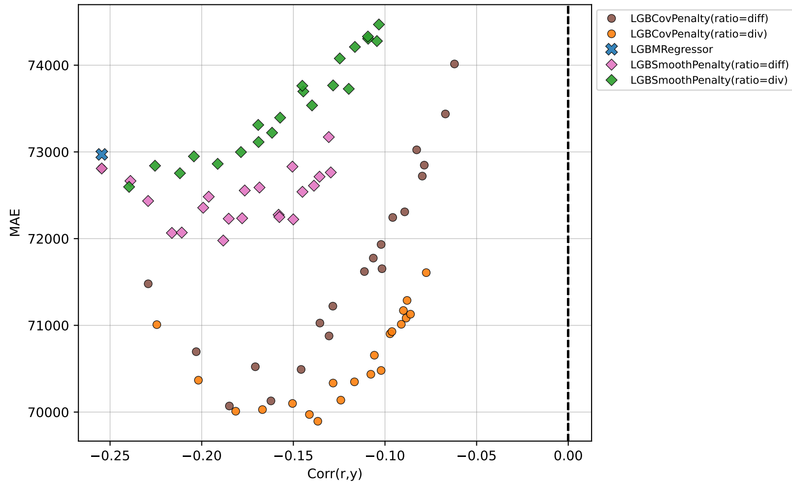
Vertical Equity Metric (Corr(r,y)) vs Error (MAE) for Different Penalization Levels [Validation Set]
