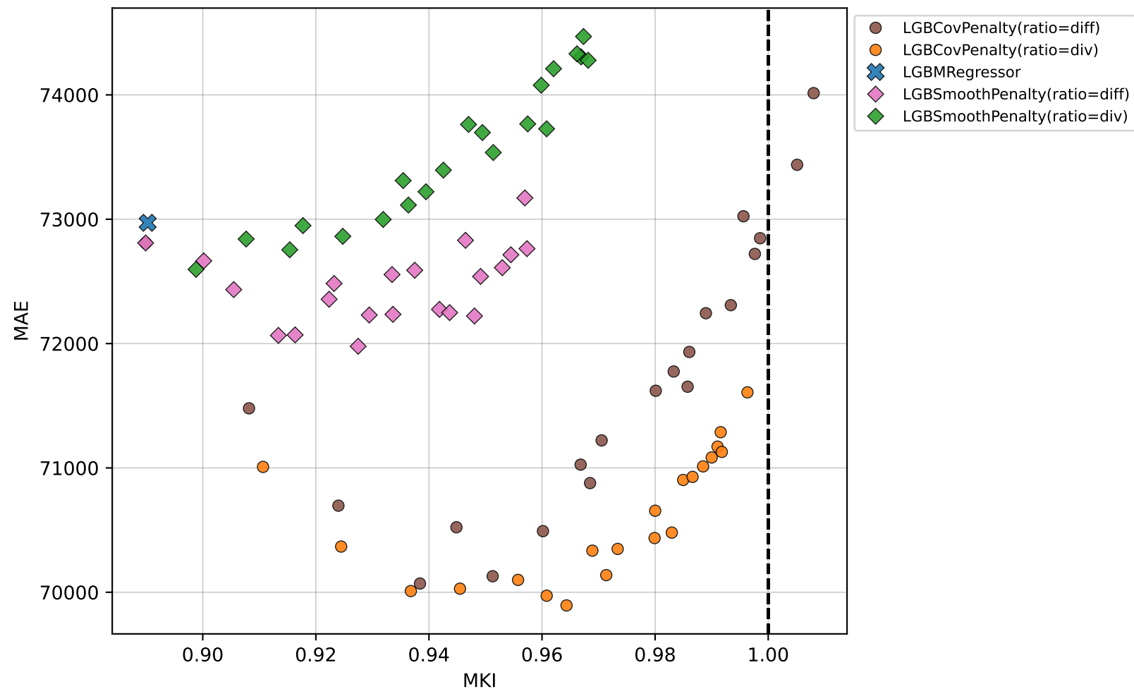
Vertical Equity Metric (MKI) vs Error (MAE) for Different Penalization Levels [Validation Set]
