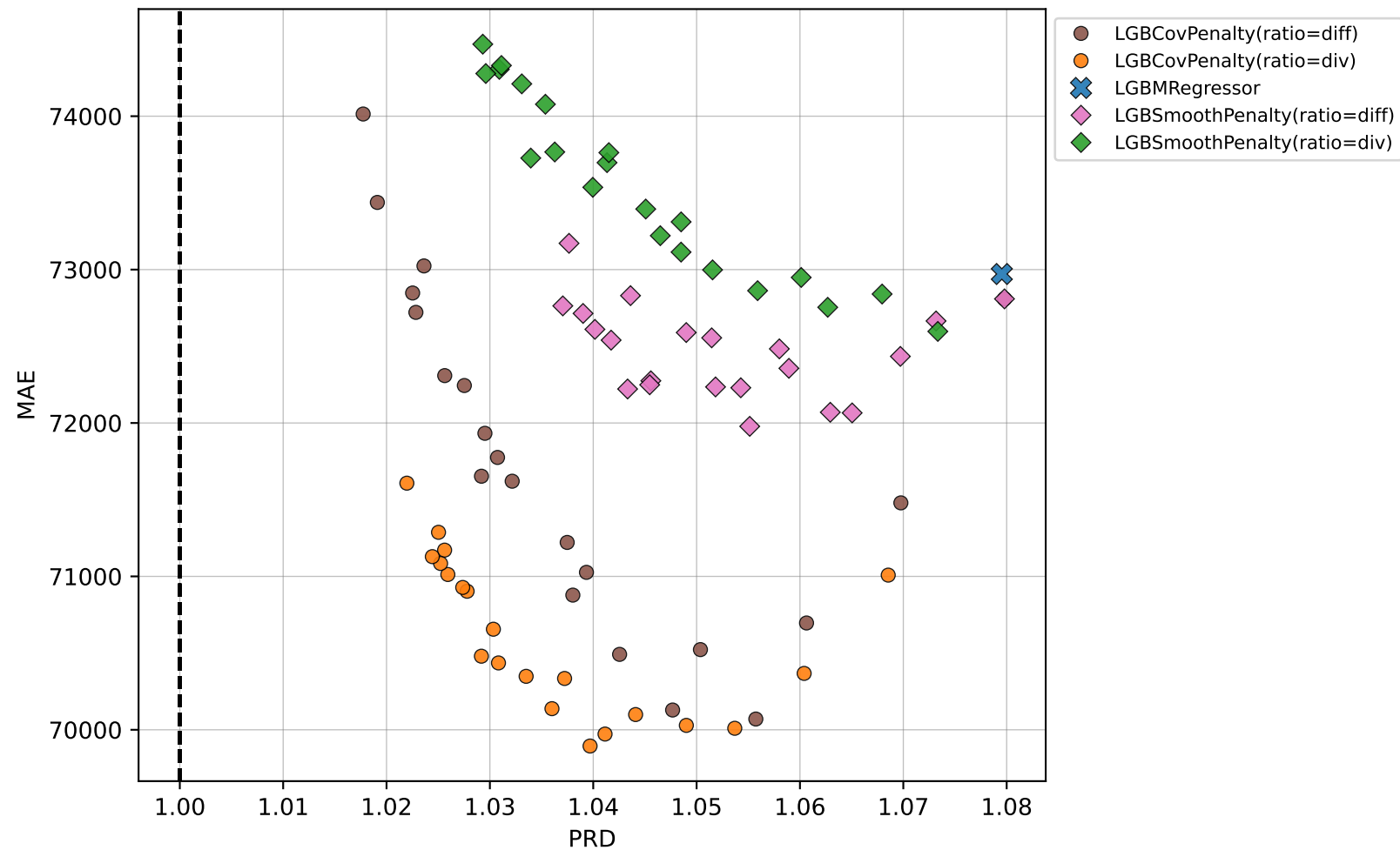
Vertical Equity Metric (PRD) vs Error (MAE) for Different Penalization Levels [Validation Set]
