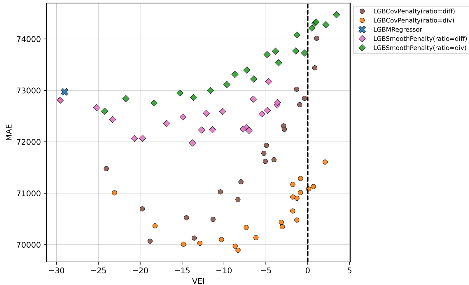
Vertical Equity Metric (VEI) vs Error (MAE) for Different Penalization Levels [Validation Set]
