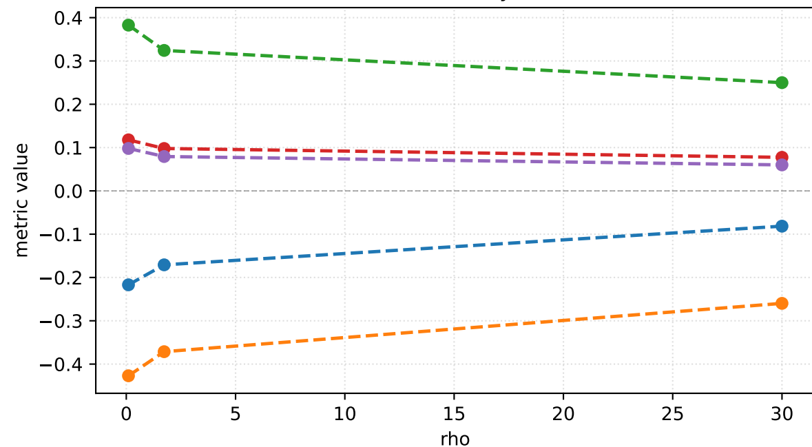
LGBCovPenalty[diff]
