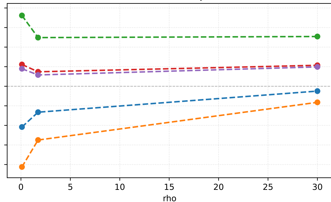
LGBSmoothPenalty[diff]
