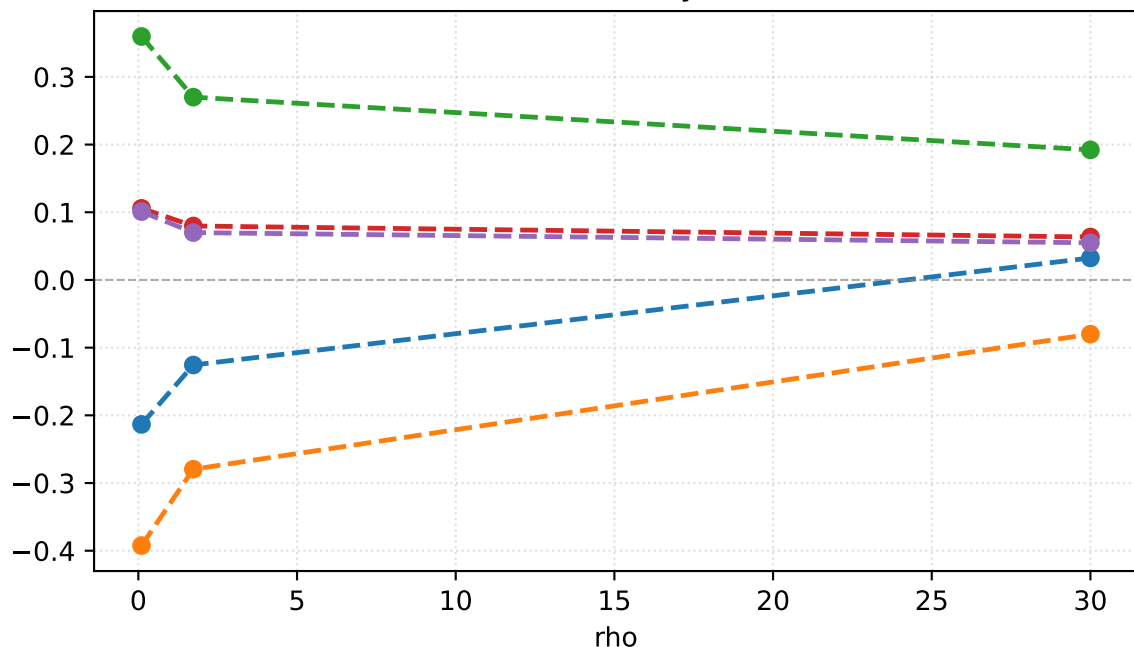
LGBCovPenalty[diff]
