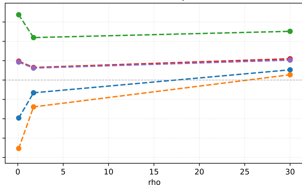
LGBSmoothPenalty[diff]
