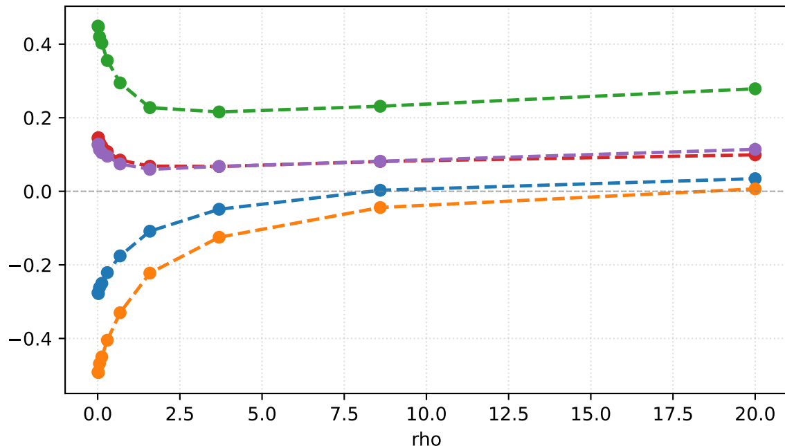
LGBSmoothPenalty
