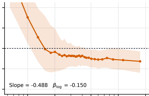
Unpenalized LightGBM
